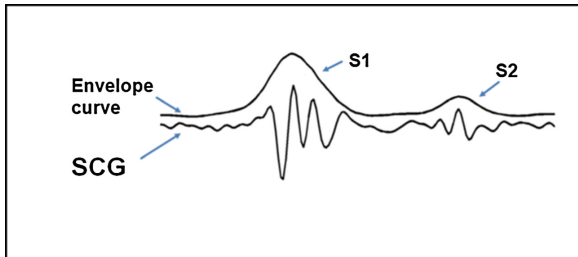
Fig. 4. SCG profile and the corresponding envelope curve
