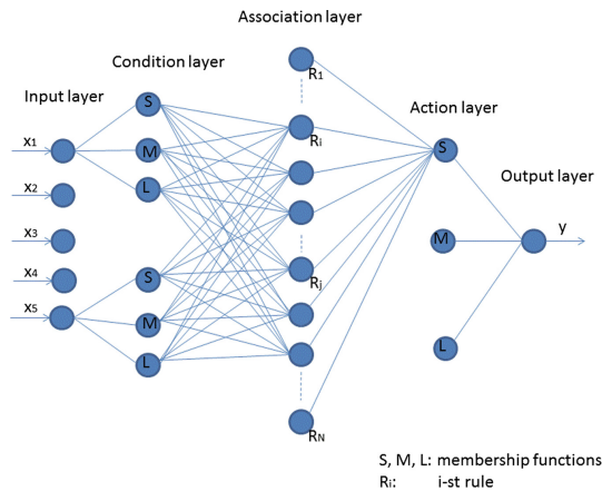
Fig. 5. EfuNN is a five layers artificial neural network where each layer corresponds to a layer of a fuzzy logic engine.
