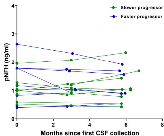
Figure 2. Longitudinal evaluation of CSF pNFH in C9ORF72 repeat expansion carriers and non-carriers. pNFH levels were measured in CSF collected longitudinally from C9ORF72 repeat expansion carriers and non-carriers. Subjects are color-coded based on their disease progression score, with patients having a score higher than the median (0.54 and 0.45 for C9ORF72 expansion carriers and non-carriers, respectively) considered faster progressors, while those with a score equal to or lower than the median considered slower progressors. (A) Among the expansion carriers, 10 were asymptomatic, 20 were patients with c9ALS, and 7 were patients with c9ALS and comorbid FTD. For these 37 subjects, the median length of time between the first and last pNFH measurement was 12.9 months (Range: 4.4– 22.6 months); 25 subjects had 2 measurements, 9 subjects had 3 measurements, 2 subjects had 4 measurements, and 1 subject had 5 measurements. (B) For the 17 ALS patients without a C9ORF72 expansion, the median length of time between the first and last pNFH measurement was 5.8 months (Range: 3.0 – 6.7 months), and CSF pNFH was measured either 2 times (N=2) or 3 times (N=15).
