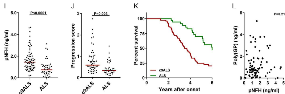
Figure 1. Evaluation of CSF pNFH in C9ORF72 repeat expansion carriers and non-carriers. pNFH levels were measured in CSF from individuals with a C9ORF72 repeat expansion (panels A–D), and those without an expansion (panels E–H). (A) Scatter plot showing that CSF pNFH levels were higher in patients with c9ALS with or without comorbid FTD (c9ALS±FTD, N=86), or patients with c9FTD (N=21), compared to asymptomatic C9ORF72 repeat expansion carriers (c9ASX, N=28). Patients with c9ALS-FTD are represented by green circles. (B) ROC curves showing the ability of CSF pNFH levels to discriminate between patients with c9ALS or c9ALS-FTD (N=86) and either asymptomatic C9ORF72 repeat expansion carriers (N=28) or patients with c9FTD (N=21). (C) Association of CSF pNFH levels and disease progression scores in patients with c9ALS or c9ALS-FTD (N=63). (D) Survival after disease onset according to CSF pNFH levels for c9ALS and c9ALS-FTD patients (N=81). For ease of presentation, pNFH levels were divided into a three-level categorical variable based on sample tertiles (Low: \leq 1.0980 ng/ml, Moderate: 1.0981–1.6860 ng/ml, High: > 1.6860 ng/ml). (E) Scatter plot showing that CSF pNFH levels among individuals without a C9ORF72 repeat expansion were higher in ALS patients with or without comorbid FTD (N=45) compared to healthy individuals (N=37) or patients with FTD (N=25). Patients with ALS-FTD are represented by green circles. (F) ROC curves showing the ability of CSF pNFH levels to discriminate between patients with ALS or ALS-FTD
