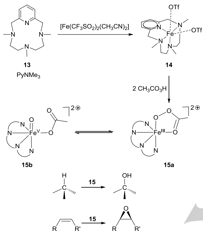
Scheme 6. Synthesis of \text{Fe}^{\text{II}} complex 14 and oxidation products 15a-b obtained upon treatment with peracetic acid. C-H hydroxylation and epoxidation catalysed by oxidant 15 .
