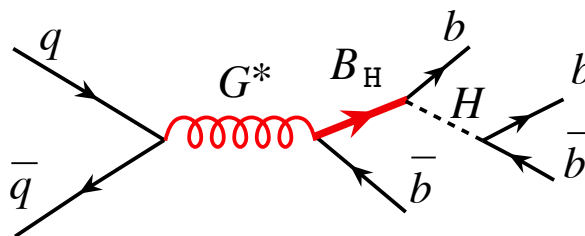
Figure 1: Feynman diagram of the signal process q\bar{q} \rightarrow G^* \rightarrow B_H\bar{b} \rightarrow Hb\bar{b} \rightarrow b\bar{b}b\bar{b} .
