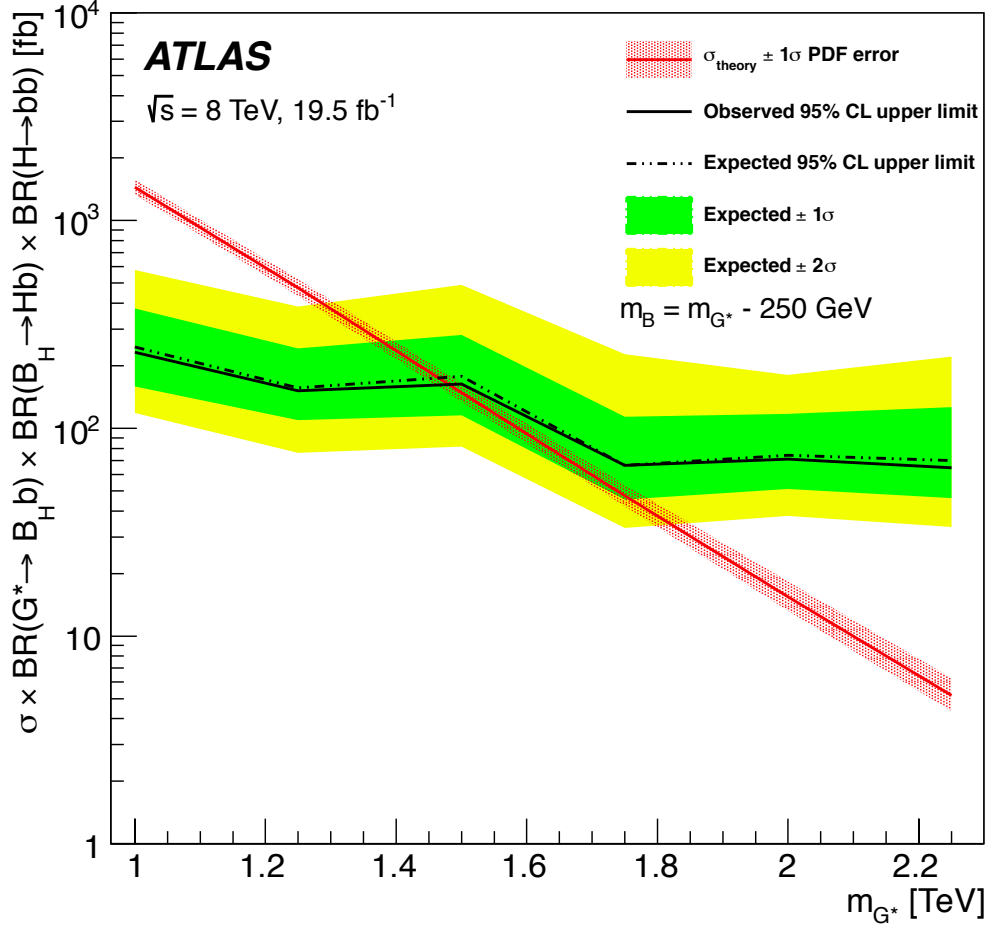
Figure 4: Observed (solid) and expected (dashed) 95% C.L. upper limits on the cross section \sigma(pp \rightarrow G^* \rightarrow B_H b) \times \text{BR}(B_H \rightarrow Hb) \times \text{BR}(H \rightarrow b\bar{b}) for VLQ mass points with m_{B_H} = m_{G^*} - 250 GeV, from the combined merged and resolved analyses, as well as the theoretical prediction based on parameters given in Section 3. The uncertainty band around the theory cross section reflects the uncertainty in the CTEQ6.6 PDFs.
