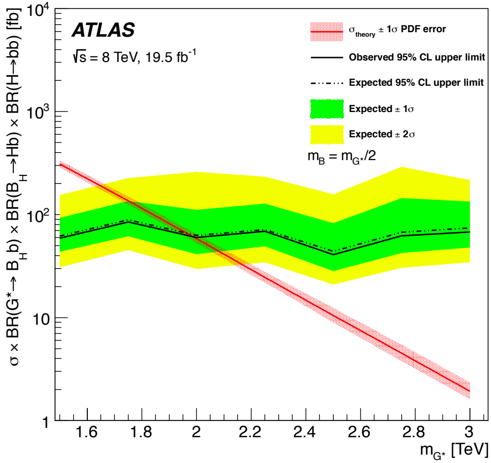
Figure 3: Observed (solid) and expected (dashed) 95% C.L. upper limits on the cross section \sigma(pp \rightarrow G^* \rightarrow B_H b) \times BR(B_H \rightarrow Hb) \times BR(H \rightarrow b\bar{b}) for VLQ mass points with m_{B_H} = m_{G^*}/2 , from the combined merged and resolved analyses, as well as the theoretical prediction based on parameters given in Section 3. The uncertainty band around the theory cross section reflects the uncertainty in the CTEQ6.6 PDFs.
