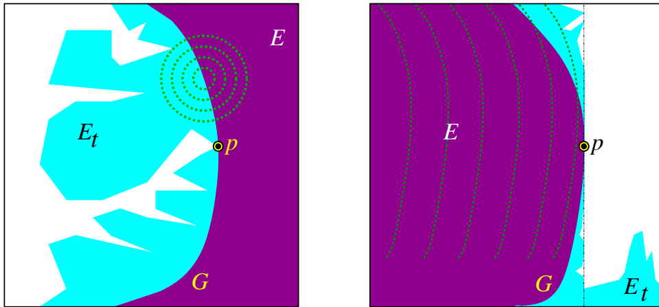
FIGURE 4. Touching \partial E_t , according to the alternative in (4.21) and (4.22).
