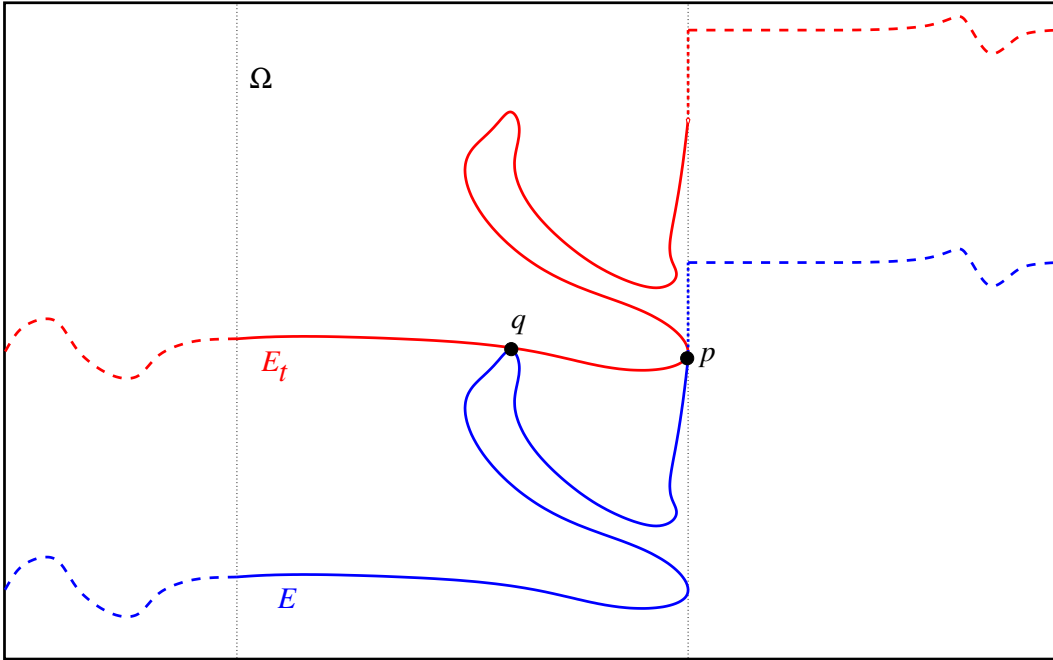
FIGURE 2. The case in (4.8).
