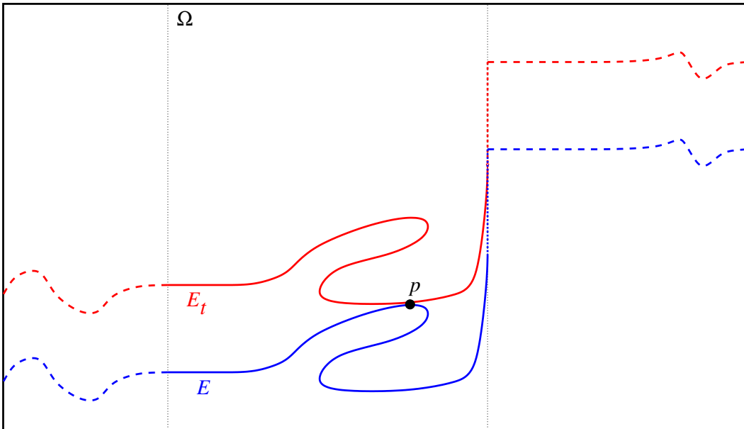
FIGURE 1. The case in (4.7).
