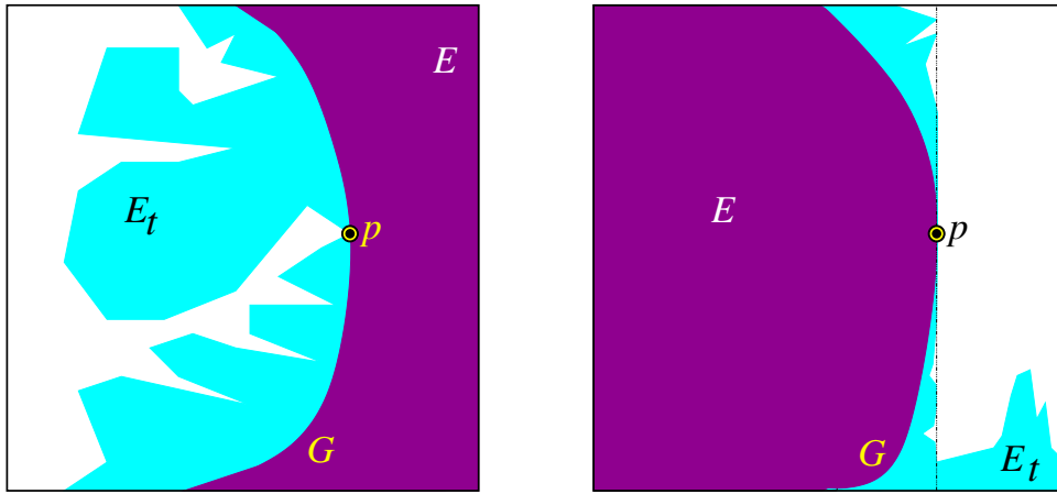
FIGURE 3. The alternative in (4.21) and (4.22).
