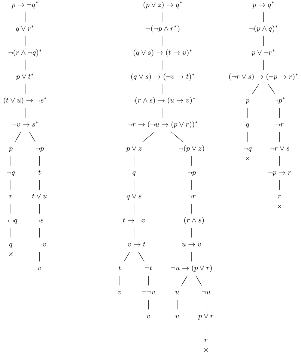
Figure 3: Intelim trees using unsigned formulae.
