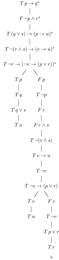
Figure 2: An intelim proof of depth 2 using S-formulae. Each branch is an intelim sequence for the set of S-formulae containing the initial assumptions (marked with *) and the virtual assumptions introduced by the applications of PB.
