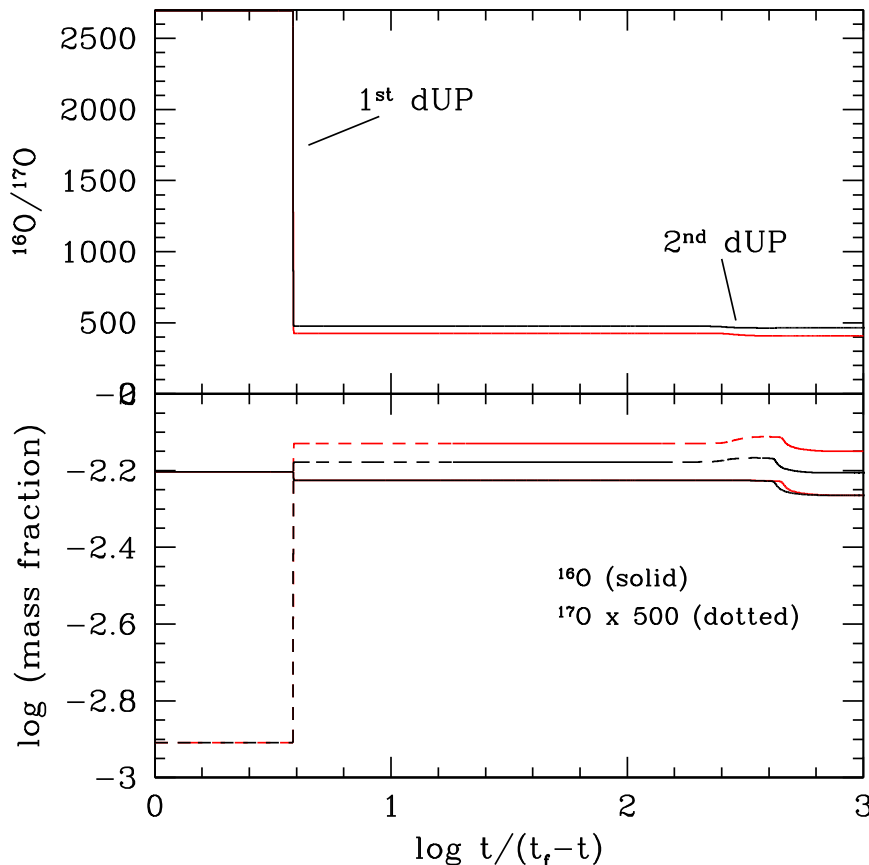
Fig. 4. Evolution of the two lighter oxygen isotopes in a 6 M_{\odot} model (solar initial composition). Upper panel: ^{16}\text{O}/^{17}\text{O} ratio. Lower panel: ^{16}\text{O} (solid) and ^{17}\text{O} (dotted). Red lines refer to the models calculated by adopting the Iliadis et al. (2010) rate for the ^{17}\text{O}(p, \alpha)^{14}\text{N} reaction, while black lines represent models obtained with the new LUNA rate (Bruno et al. 2016). t_f = 68 Myr corresponds to the age of the last computed model (end of the early AGB).
