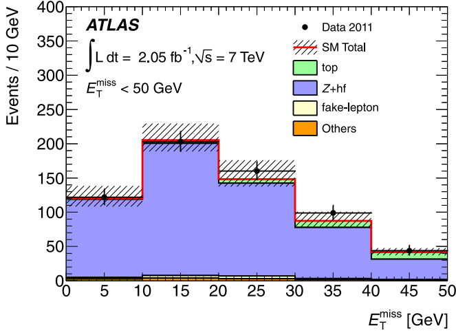
Fig. 2. The distribution of E_T^{\text{miss}} for the Z+hf validation region for the sum of ee and \mu\mu channels. By construction, only events with E_T^{\text{miss}} below 50 GeV are displayed. The dashed band represents the experimental uncertainties including effects due to JES, b -tagging and lepton ID efficiency.
