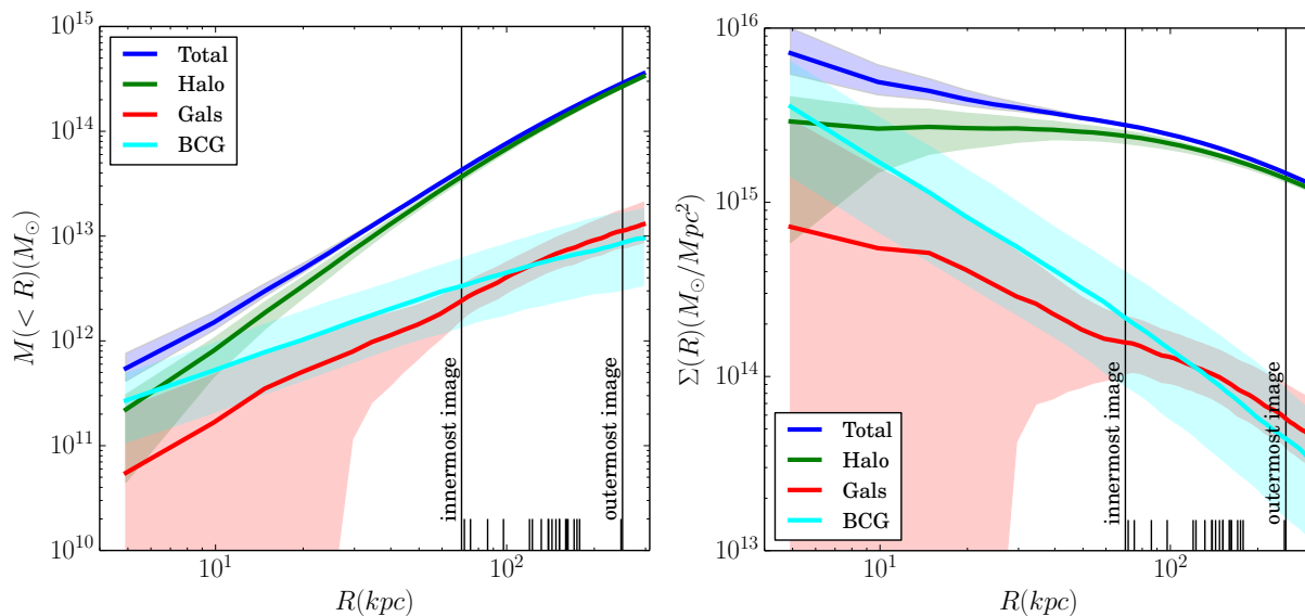
Figure 1. Projected mass, M(< R) , and surface mass density \Sigma(R) relatively to the BCG center for the total, cluster dark-matter (Halo), galaxy members (Gals) and BCG mass components. The solid lines represent the median and the filled contours the 68% confidence level from the strong lensing total mass reconstruction. The vertical lines show the positions of the multiple images.
