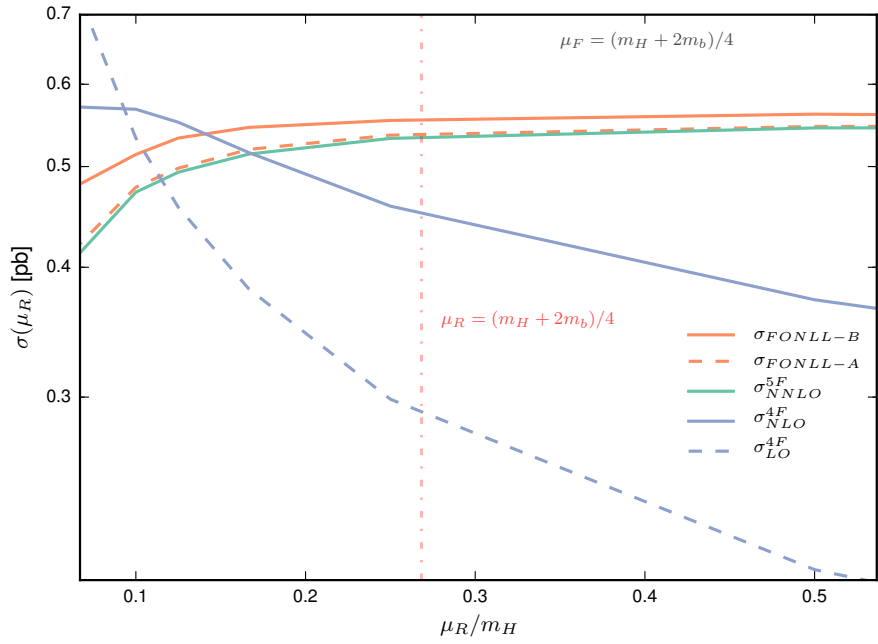
Figure 2: Comparison of the FONLL matched result and its 4FS and 5FS components, Eq. (1). Results are shown as a function of the renormalization scale, with the factorization scale fixed at a high value \mu_F = m_H (top) or a low value \mu_F = \frac{(m_H + 2m_b)}{4} (bottom).
