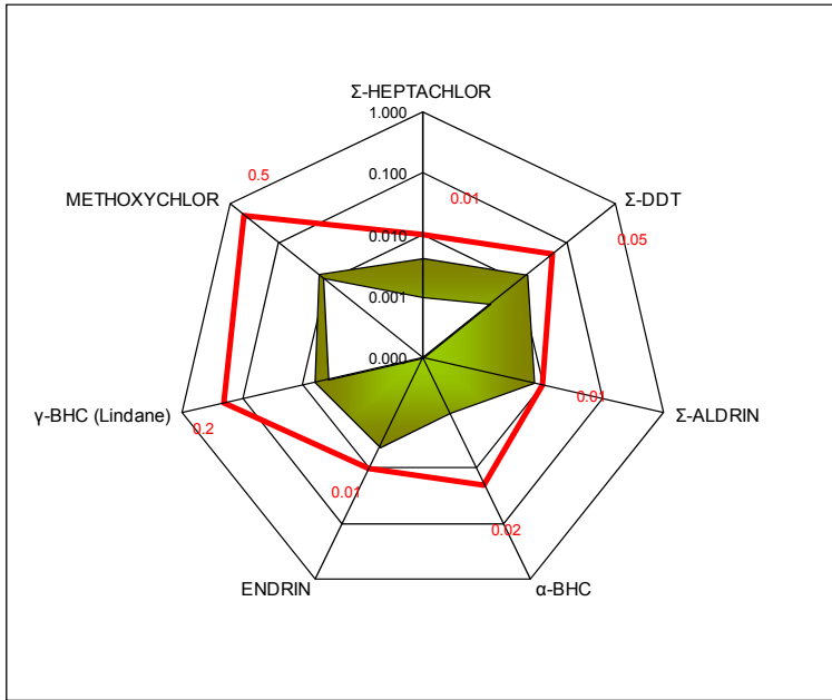
Figure 8. Radar plot of detected OCPs content in (mg kg -1 ) feed samples in relation to MRLs (red line)
