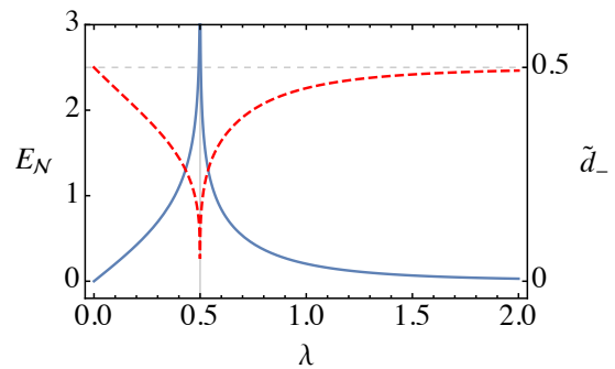
FIG. 1: (Color online) Plot of the logarithmic negativity E_N(\lambda) (blue solid curve) and of the lowest symplectic eigenvalue \tilde{d}_-(\lambda) (red dashed curve) of the partially transposed CM. The dashed gray line at \tilde{d}_- = 0.5 represents the threshold of separability, under which the state is entangled. Parameters: \omega = \omega_0 = 1 and \lambda_c = 0.5 (gray vertical line), in units of \omega_0 .
