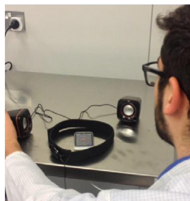
Figure 3: Testing setup.
