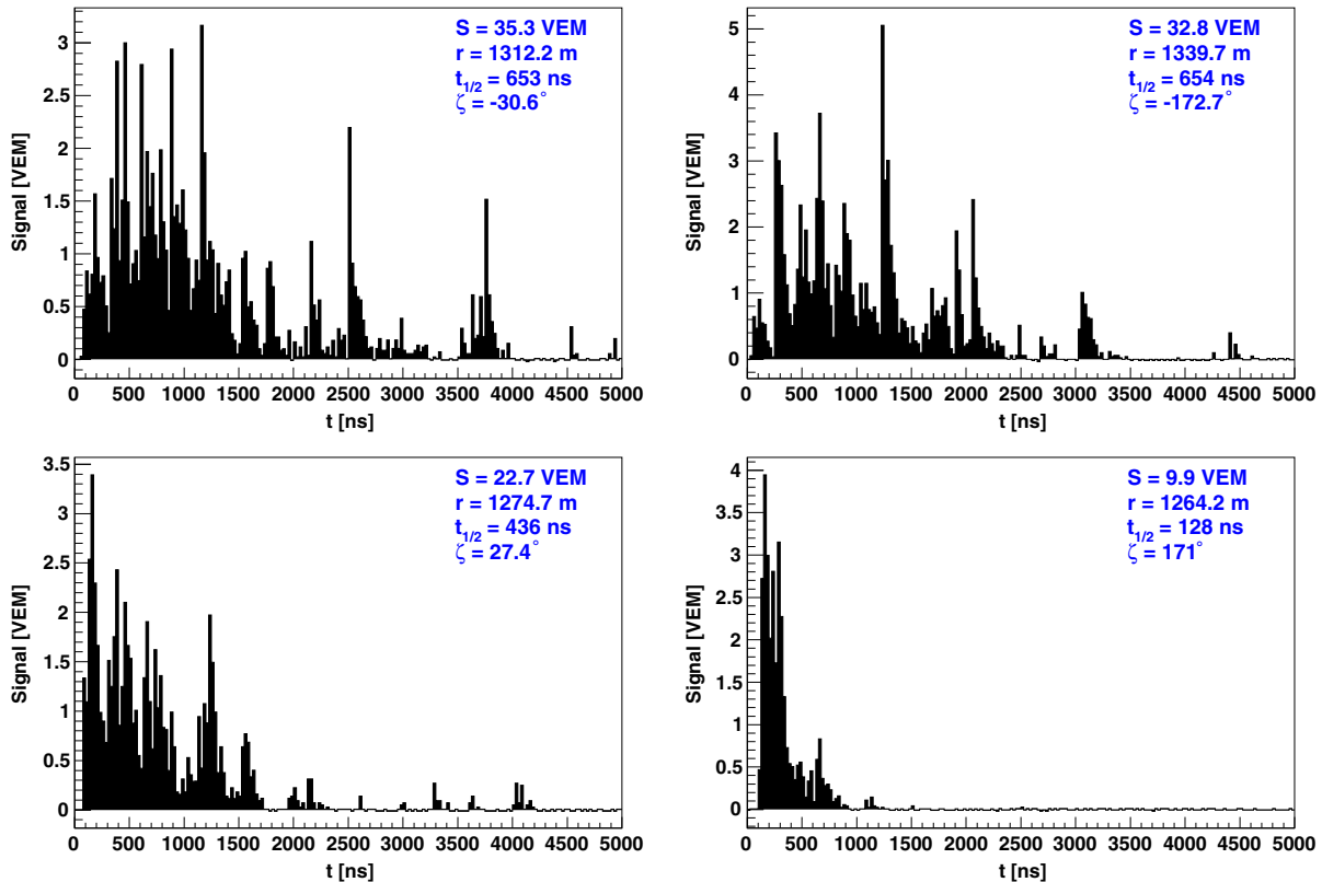
FIG. 2. Top: two stations in an event of 16.9 \text{ EeV} and 15.7^\circ in zenith. Bottom: two stations in an event of 7.7 \text{ EeV} and 52^\circ in zenith. Left panels correspond to early stations while right panels correspond to late stations.
