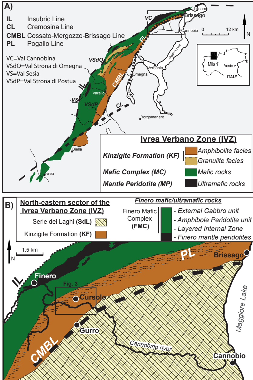
Figure 1. A) Sketch map of the Ivrea-Verbania Zone (westernmost part of the southern Alps) simplified after Zingg et al. (1990) and Boriani et al. (1990). Black box delimits the northeastern-most part of the IVZ. B) Schematic geological map of the north-eastern sector of the IVZ, modified after Boriani et al. (1990). Black box delimits the studied area which geological sketch map is shown in Figure 3.
