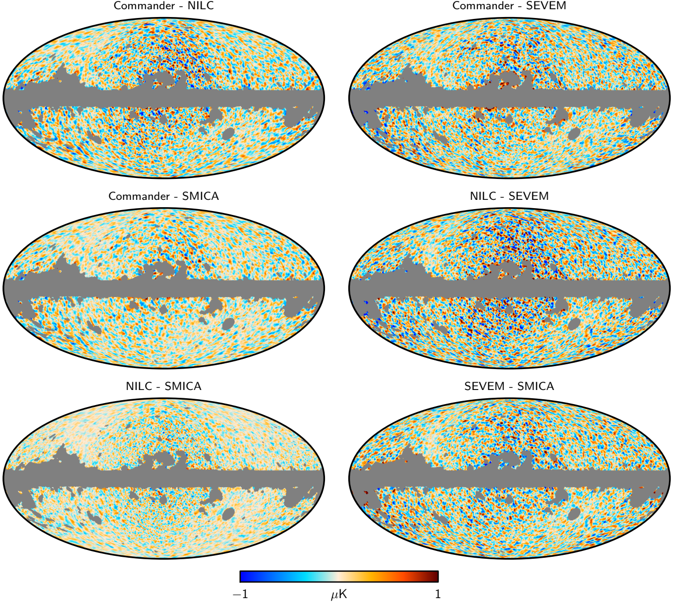
Fig. 10. Pairwise differences between CMB U maps, after smoothing and downgrading as in Fig. 9.
