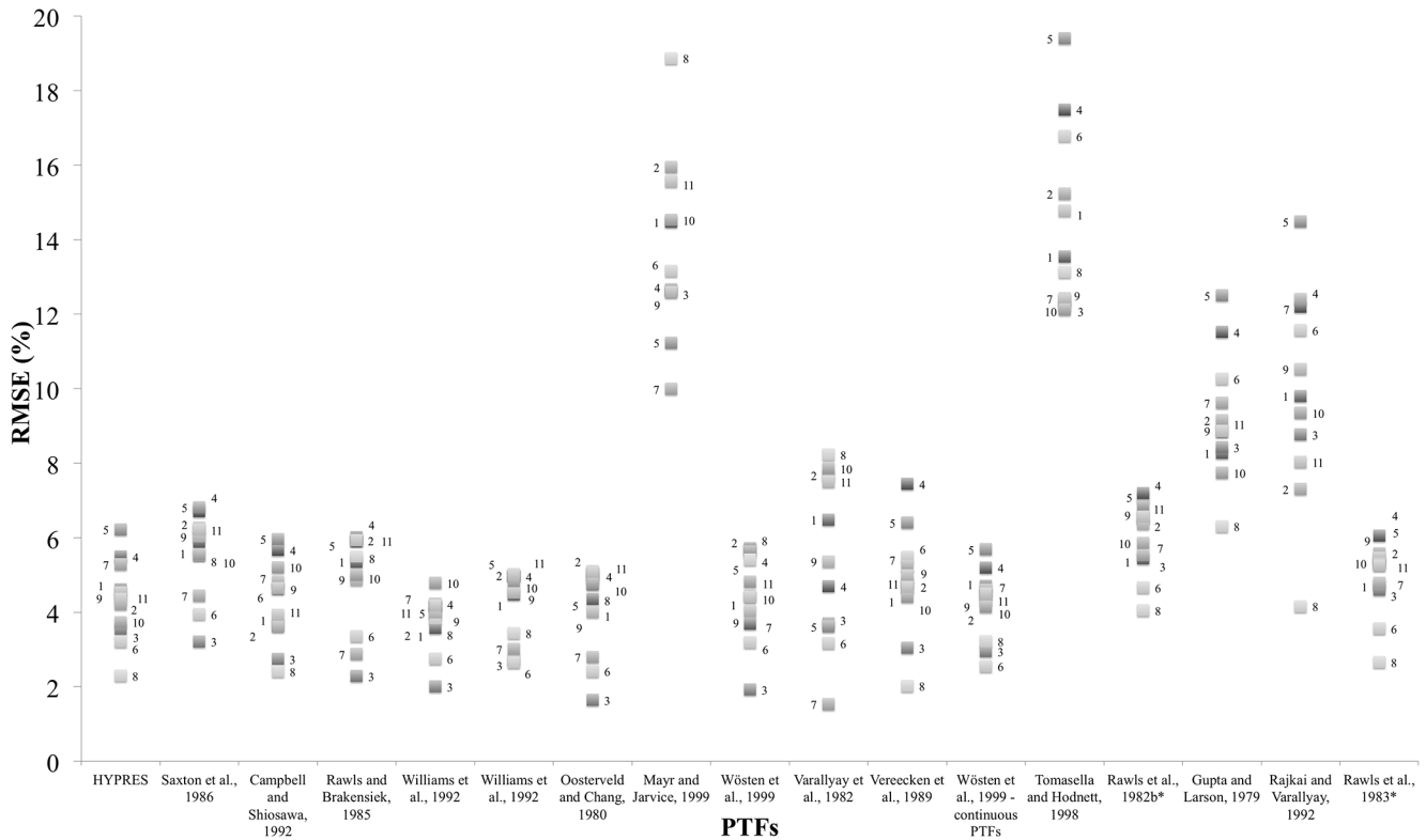
Figure 3. Matrix representing the result of the RMSE test – each pixel for a combination of the soil’s PTF and RMSE.
