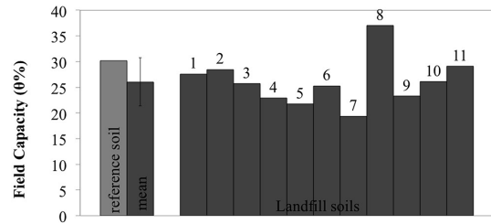
Figure 6. Volumetric water content ( \theta %) at field capacity: comparison between reference soil and landfill soils.
