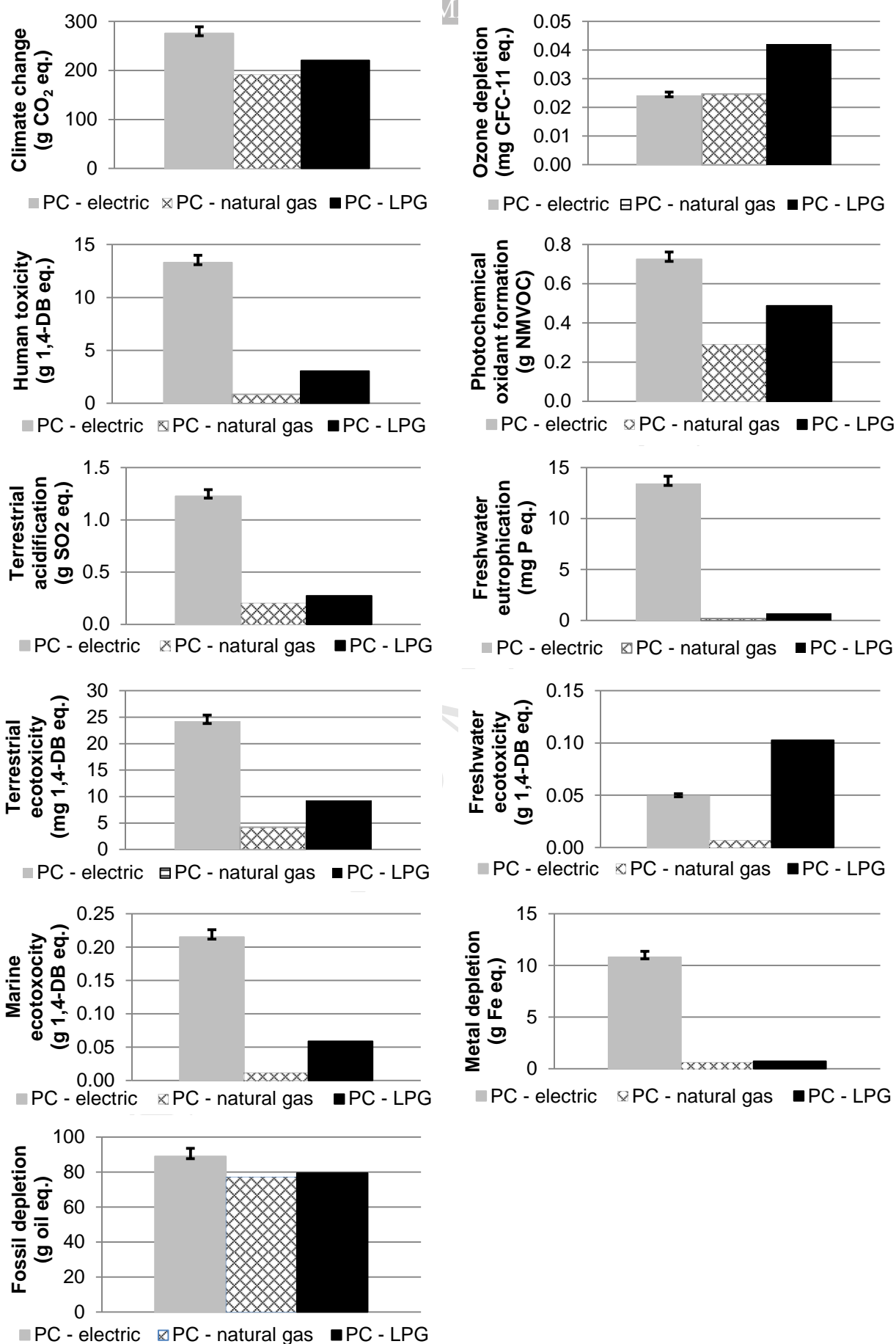
Figure 4 Environmental impacts of cooking in different types of pasta cooker (PC)
