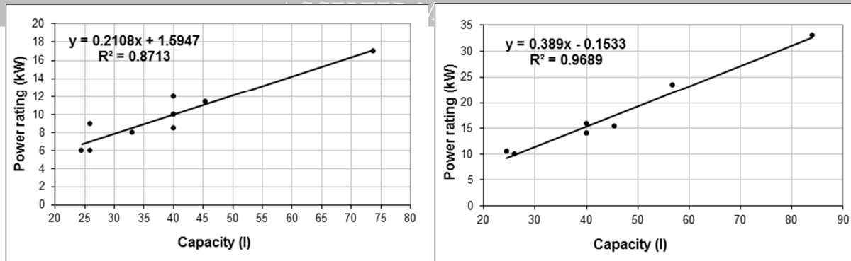
a) Electric pasta cookers
