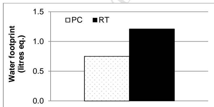
Figure 8 Water footprint of cooking for pasta cookers (PC) and range tops (RT).
