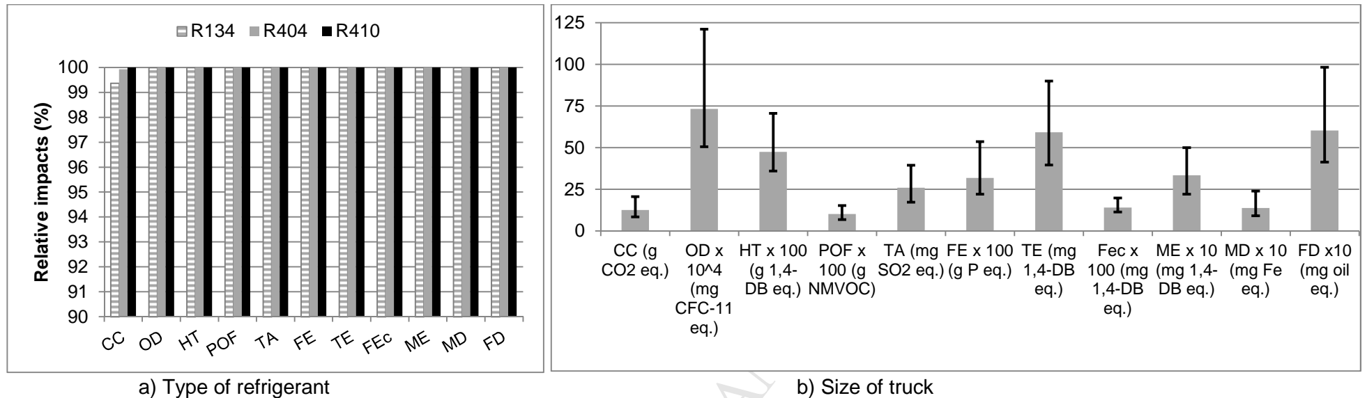
Figure 11 The relative impacts of refrigerated transport using different refrigerants and the effect on the impacts of the size of truck. [For impacts nomenclature, see Figure 5. The results refer to a distance of 50 km.]
