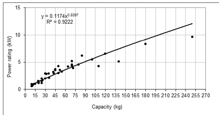
Figure 3 The relationship between the capacity and power rating of blast chillers estimated using data from manufacturers.
