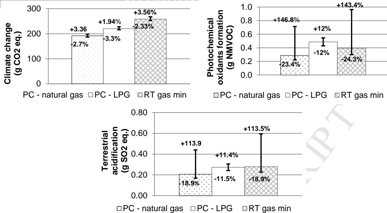
Figure 7 Environmental impacts of pasta cookers (PC) and range tops (RT) for the three categories affected by the changes in emissions from natural gas.
