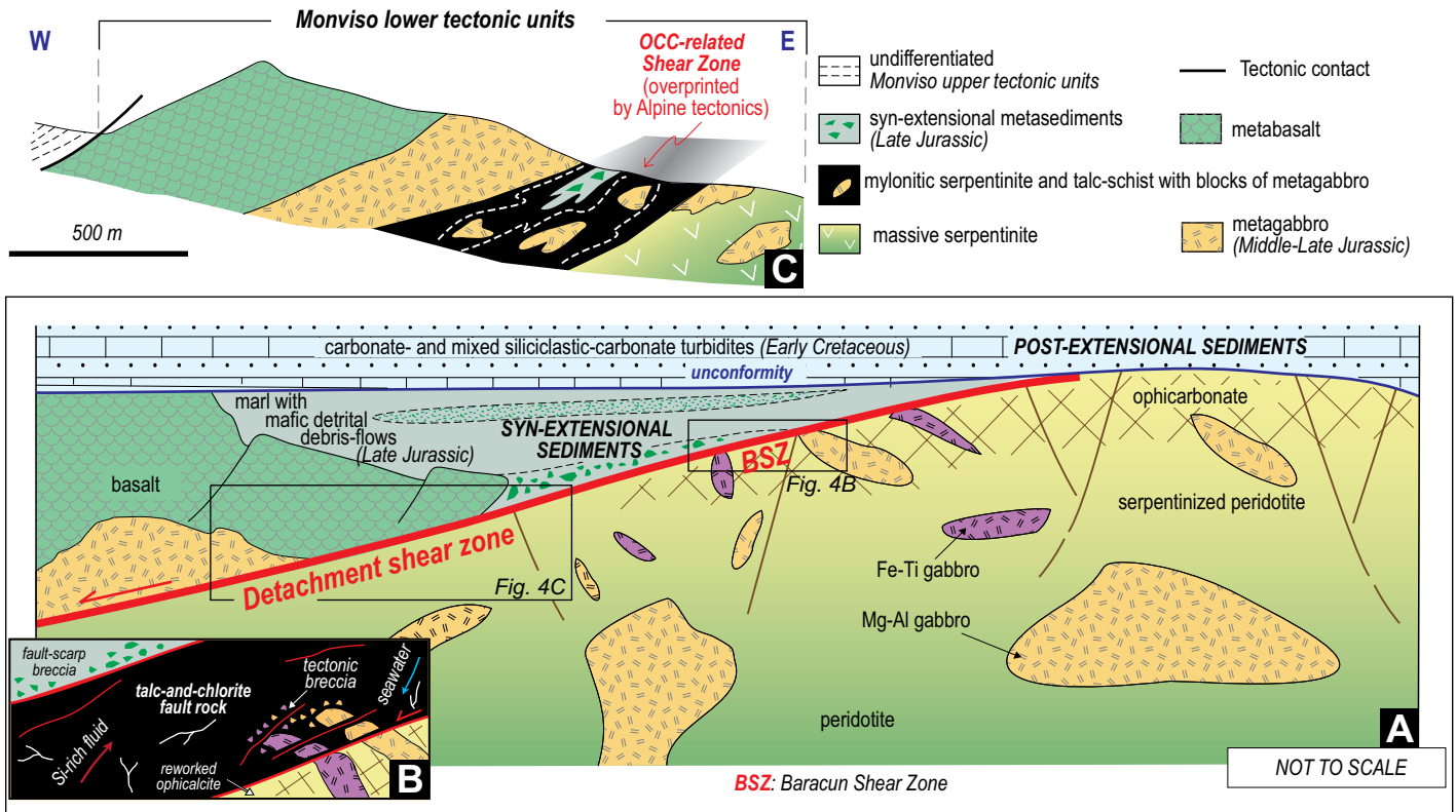
Figure 4. (A) Interpretive cross section for the development of the oceanic core complex (OCC), Baracun shear zone and syn- and postextensional sequences in the Monviso ophiolite. (B) Close-up of the Baracun shear zone, depicting the inferred tectonic and hydrothermal processes. (C) Close-up of the representative cross section of Figure 1C, depicting at a regional scale the prolongation of the Baracun shear zone within the Monviso ophiolite lower tectonic units.
