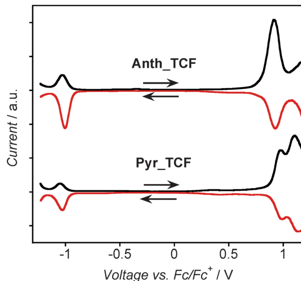
Fig. 4 Differential pulse voltammetry of Anth_TCF (top) and Pyr_TCF (bottom) recorded in \text{CH}_2\text{Cl}_2 solution containing 0.1 M [TBA][PF 6 ] and referenced to ferrocene. Arrows indicate the direction of scan.
