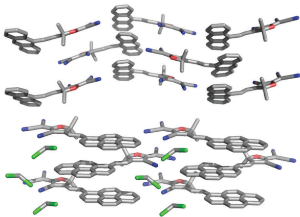
Fig. 3 Crystal packing of Anth_TCF (top) and Pyr_TCF (bottom). Hydrogens have been omitted for clarity.
