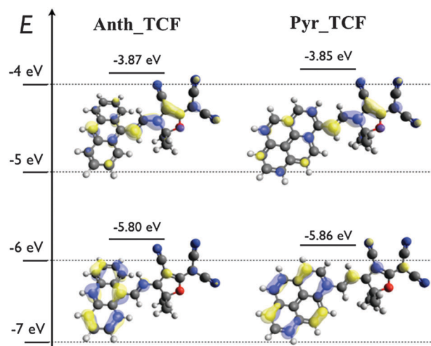
Fig. 6 Molecular orbital distribution of HOMO (bottom) and LUMO (top) of Anth_TCF and Pyr_TCF at B3LYP/6-31G(d) level of theory (isodensity = 0.04). Absolute HOMO and LUMO energy levels are experimentally obtained from electrochemical means following the equation E_{\text{HOMO/LUMO}} (eV) = -4.88 - E_{\text{OX/RED}} (V vs. Fc/Fc + ). 48
