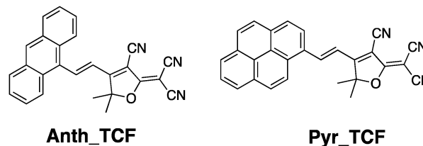
Fig. 1 Chemical structures of TCF derivatives used in this study.
