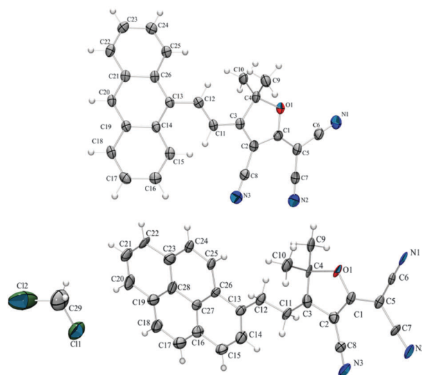
Fig. 2 ORTEP drawings of Anth_TCF (top) and Pyr_TCF (bottom) with thermal ellipsoids drawn at the 50% probability level.
