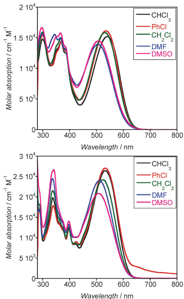
Fig. 5 UV-Visible absorption spectra of Anth_TCF (top) and Pyr_TCF (bottom) in various solvents acquired at 5 \times 10^{-5} M.
