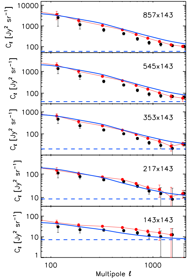
Fig. 16. CIB cross- and auto- power spectra obtained at 143 GHz (red points). To obtain the CIB, the cleaned CMB and Galactic dust power spectra (black points, shifted in l for clarity) are corrected for SZ-related residuals, C_{SZcorr}^{y \times y'} and C_{CIB-SZcorr}^{y \times y'} (following Eqs. (8), (9), and (12)), and for C_{CIBcorr}^{y \times y'} (following Eq. (4), and computed using the extrapolation of the best-fit halo model). The prediction of the halo model is shown in blue (continuous for 2h+1h+shot noise; dashed for shot noise only).
