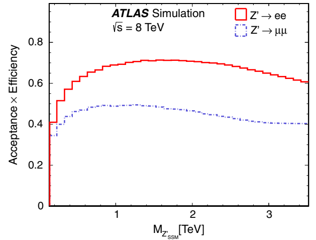
FIG. 1 (color online). Product of acceptance and efficiency for the dielectron (upper distribution) and dimuon (lower distribution) selections as a function of the Z_{\text{SSM}} pole mass.
