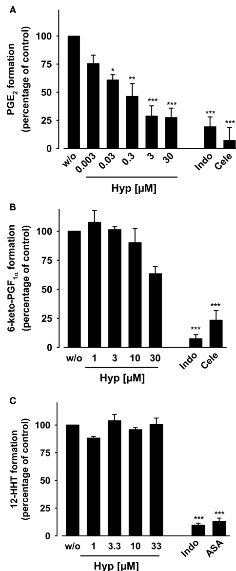
FIGURE 2 | Effects of hyperforin on arachidonic acid-induced prostanoid formation in human whole blood. (A,B) Heparinized human whole blood was treated with 10 μg ml -1 LPS for 16 h at 37°C and 5% CO 2 , supplemented with TX synthase inhibitor CV4151 (1 μM), and pre-incubated with Hyp or vehicle (DMSO) for 10 min at 37°C. (A) Then, PGE 2 formation was initiated with 20 μM AA, and PGE 2 formed within 10 min was separated by RP-HPLC and quantified by ELISA. The 100% value corresponds to PGE 2 levels in the range of 18–31 ng ml -1 in the individual experiments, respectively. (B) 6-keto PGF 1α was directly determined in the plasma by ELISA. The 100% value corresponds to 6-keto PGF 1α levels in the range of 4–7 ng ml -1 . Indomethacin (Indo, 50 μM) and celecoxib (Cele, 20 μM) were used as controls. (C) 12-HHT formation in whole blood. Heparinized whole blood was pre-incubated with Hyp or vehicle (DMSO) for 10 min, and AA (100 μM) and Ca 2+ -ionophore (30 μM) were added to induce 12-HHT product formation. After 10 min at 37°C, 12-HHT was extracted from the plasma by RP-18 solid phase extraction and analyzed by RP-HPLC as described. The 100% value corresponds to 1.5–2.4 μg ml -1 12-HHT. Indomethacin (Indo, 20 μM) and aspirin (ASA, 30 μM) were used as controls. Data are given as mean ± SE, n = 3–5, *p < 0.05, **p < 0.01 or ***p < 0.001 vs. vehicle (0.1% DMSO) control, ANOVA + Tukey HSD post hoc tests.
