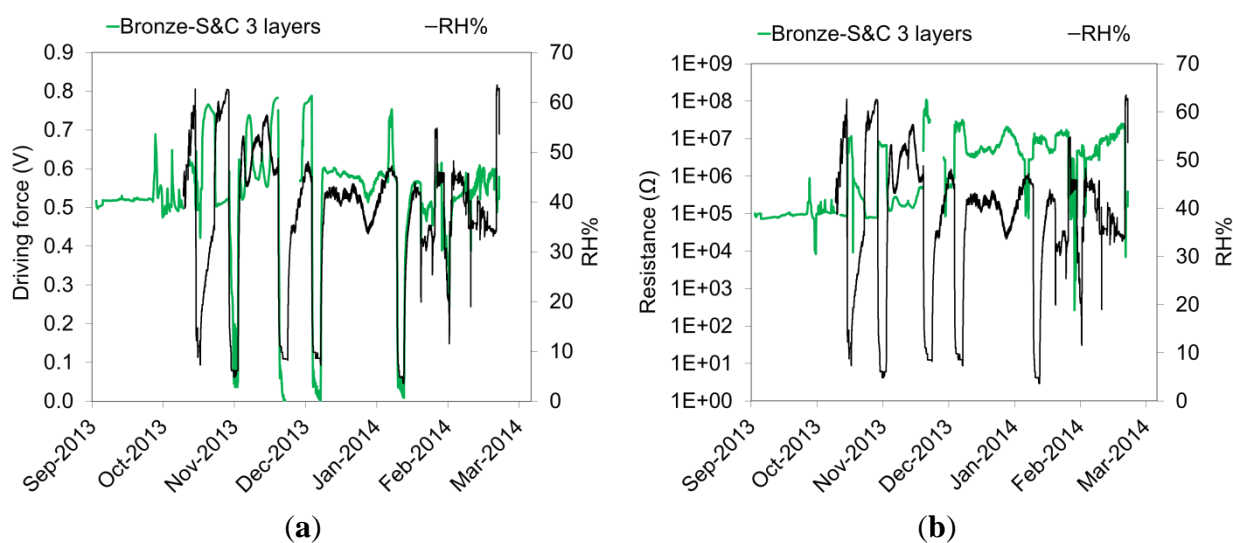
Figure 10. Driving force (a) and Resistance (b) as a function of time a galvanic sensors with bronze substrate and triple layer of S&C artificial patina.
