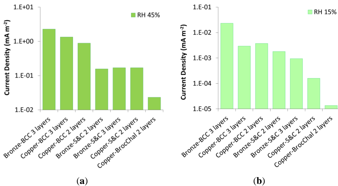
Figure 12. Average macrocouple current density as a function of the artificial patina composition and thickness, detected at constant temperature (25 °C) during the fifth month of life of the galvanic sensors at RH% 45% (a) and 15% (b).
