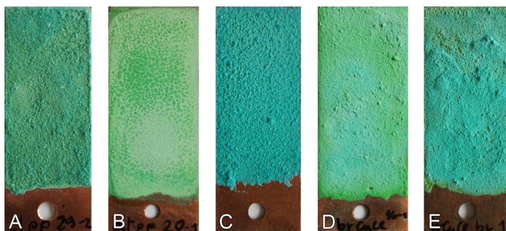
Figure 3. Photographic documentation of the different types of patina: S&C (A); BCC (B); BrocChal (C); BrocNan (D); BrocNan+Broc (E) (specimens dimensions: 60 × 20 mm).
