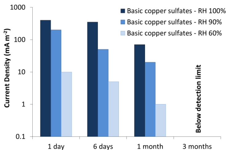
Figure 1. The galvanic sensors of the seventies [48,49]: macrocouple current as a function of time and relative humidity.
