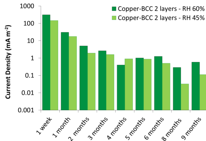
Figure 11. Average macrocouple current density detected at constant temperature (25 °C) and relative humidity (60% and 45%) for galvanic sensors with copper substrate and double layer of BCC artificial patina.
