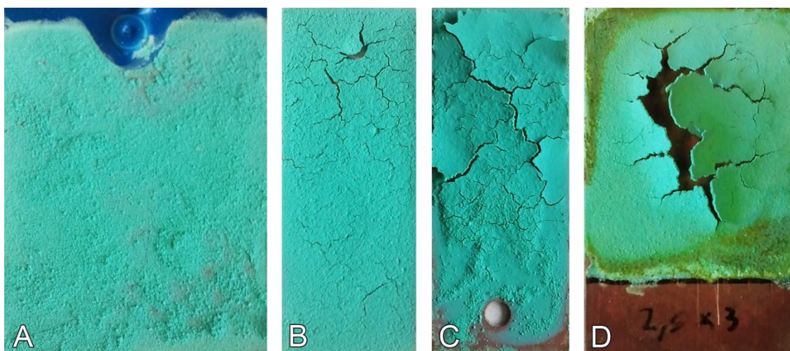
Figure 5. Brochantite patinas with increasing thickness (A) > (B) > (C) > (D) (sensors max. length: 60 mm).
