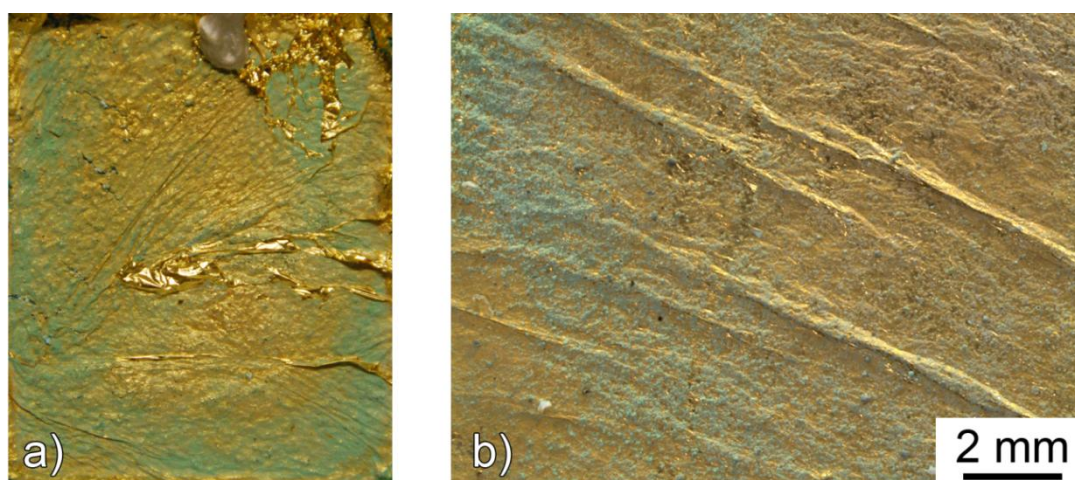
Figure 7. Macroscopic (sensor dimensions: 60 \times 50 mm) (a) and microscopic (b) documentation of a galvanic sensors resulting from the too early application of the gold leaf on a highly moistened patina.
