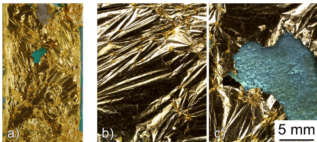
Figure 8. Macroscopic (sensors max. length: 60 mm) (a) and microscopic documentation (b,c) of a galvanic sensors showing a lack of adhesion of the gold leaf.
