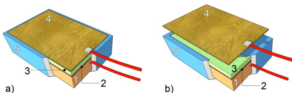
Figure 2. General model of a galvanic sensor (a) with detail of the gold leaf overlapped (b). The complete stratigraphy of the sensor includes: (1) metallic substrate; (2) cuprite layer; (3) patina of corrosion products; (4) gilding; (5) electric insulation cover.
