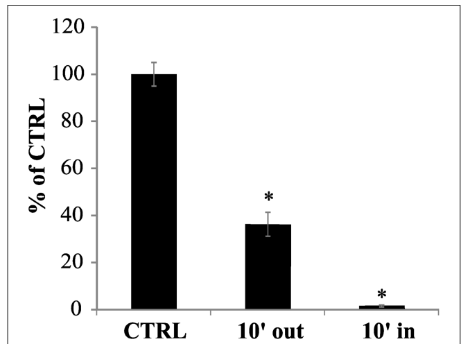
FIGURE 4 | cPTIO uptake in cell cultures. cPTIO(NNO) was incubated with cell cultures. At 10 min a sample from the culture medium was collected (10' out) and all cells were harvested. The cells were disrupted and centrifuged. An aliquot of the supernatant was collected (10' in). EPR signals were detected and given as percentage of the total signal resulting from measurement of 100 μM cPTIO(NNO) dissolved in water (CTRL) ± SD. A Student's t -test was performed and samples statistically different from the CTRL marked with an asterisk
