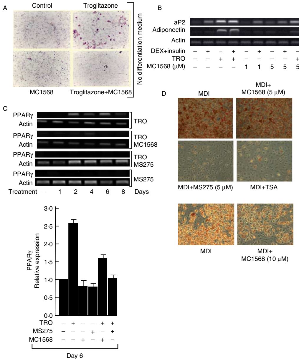
Figure 2 MC1568 attenuates TZD-induced PPAR \gamma induction and adipogenesis of 3T3-L1 cells, while pan-HDAC inhibitors block differentiation completely. (A) Morphological analysis obtained with oil red O staining and (B) RT-PCR of molecular differentiation markers in 3T3-L1 cells treated as indicated; (C) RT-PCR of PPAR \gamma expression in the 3T3-L1 cells treated as indicated; (D) morphological analysis obtained with oil red O staining of 3T3-L1 cells in complete differentiation medium and treated with TSA at 125 nM and with MS275 or MC1568 at 5 or 10 \mu M. TRO, troglitazone; DEX, dexamethasone; MDI, differentiation cocktail consisting of isobutylmethylxanthine, dexamethasone, and insulin.
