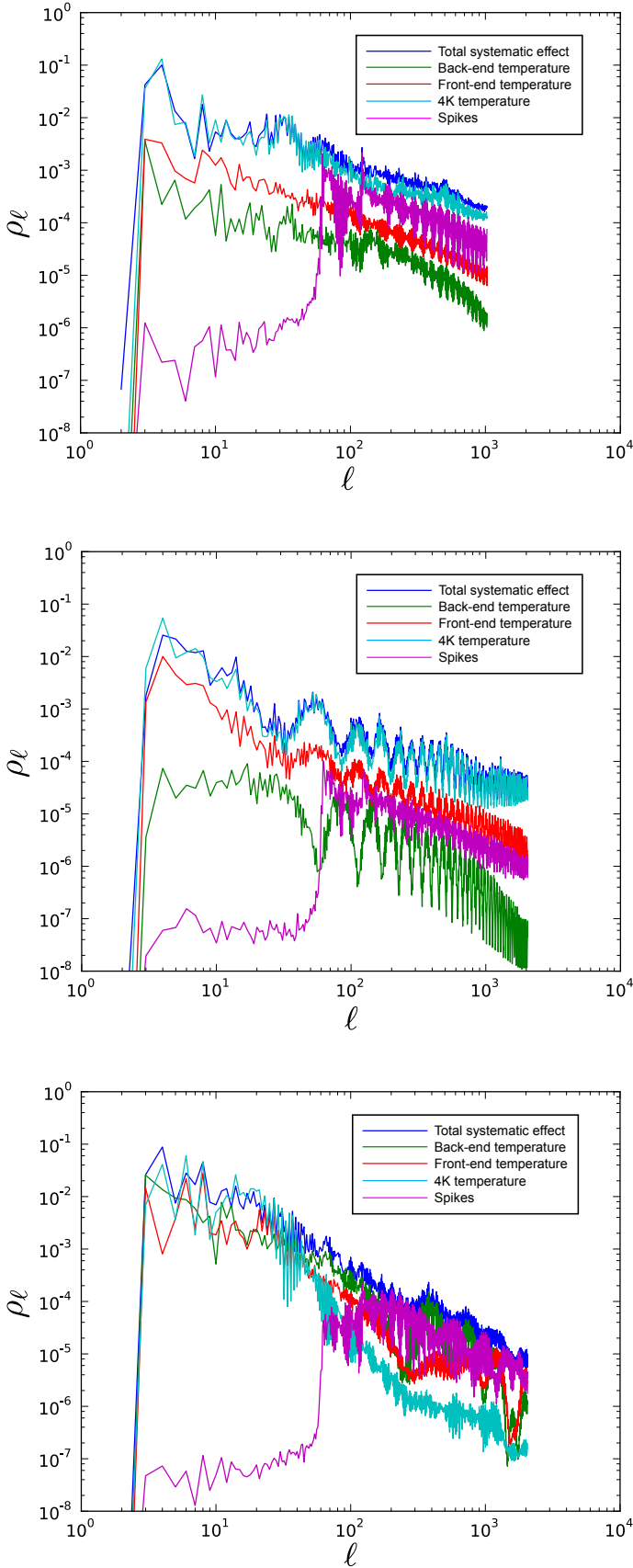
Fig. 26. Ratio \rho_\ell = C_\ell^{\text{sys}}/C_\ell^{\text{noise}} for the three LFI frequency channels (top: 30 GHz; middle: 44 GHz; bottom: 70 GHz). In each panel we have plotted both the global spectrum obtained from the maps in Fig. 25 and the individual spectra calculated from the single-component maps.
