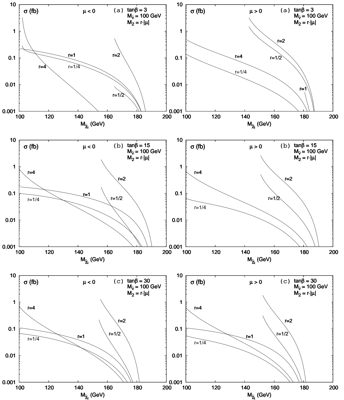
Figure 5: Total cross section for e^+e^- \rightarrow h \tilde{\chi}_1^+ \tilde{\chi}_1^- at \sqrt{s} = 500 \text{ GeV} , for \tan \beta = 3, 15, 30 , m_{A^0} = 500 \text{ GeV} , and M_{\tilde{\nu}_e} = 100 \text{ GeV} .
