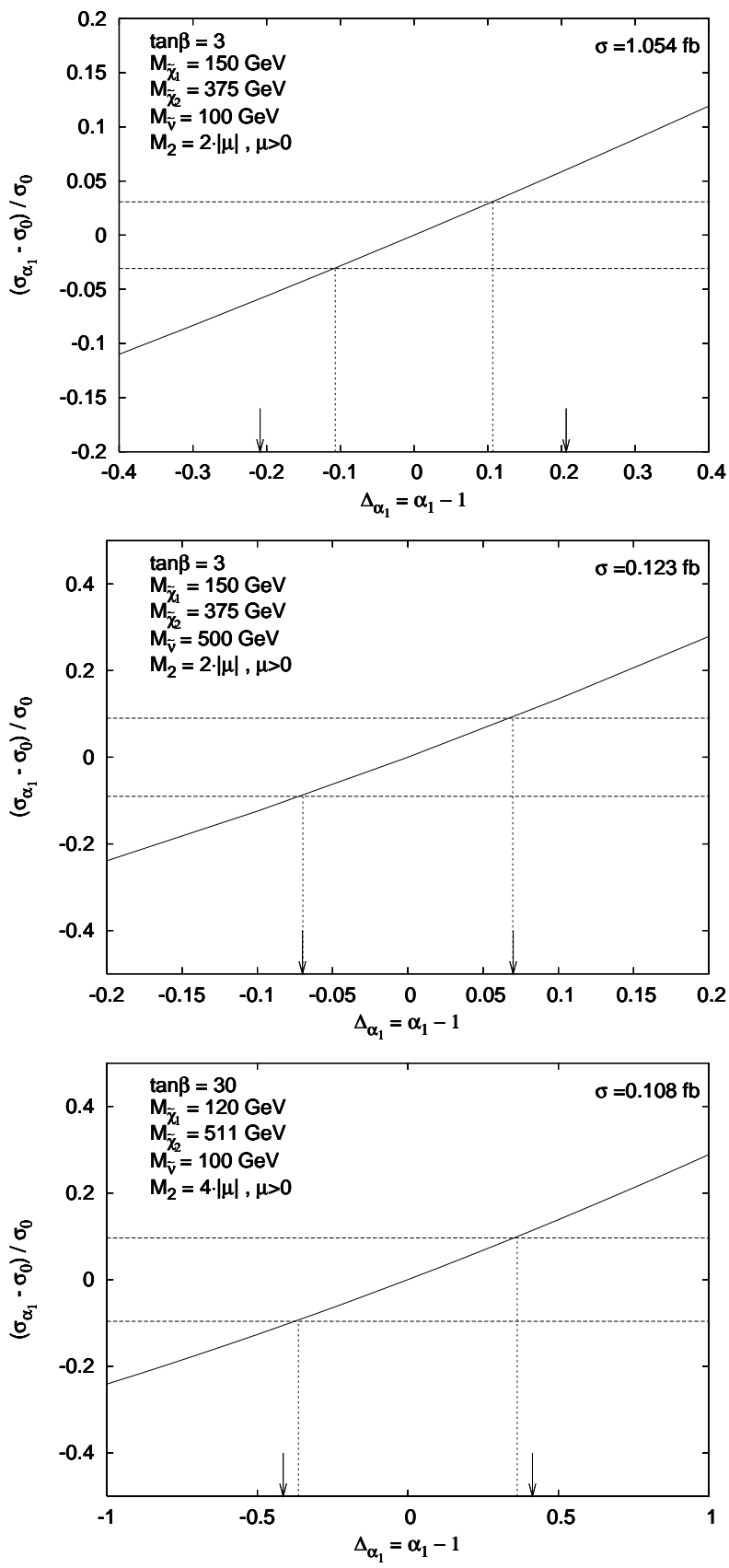
Figure 7: Relative total cross section variation for e^+e^- \rightarrow h\tilde{\chi}_1^+\tilde{\chi}_1^- at \sqrt{s} = 500 GeV, versus a change in the \alpha_1 parameter, as defined in Eq. (10), in three different scenarios. Arrows show the effect of a 3 % error on the h\tilde{\chi}_1^+\tilde{\chi}_2^- determination.
