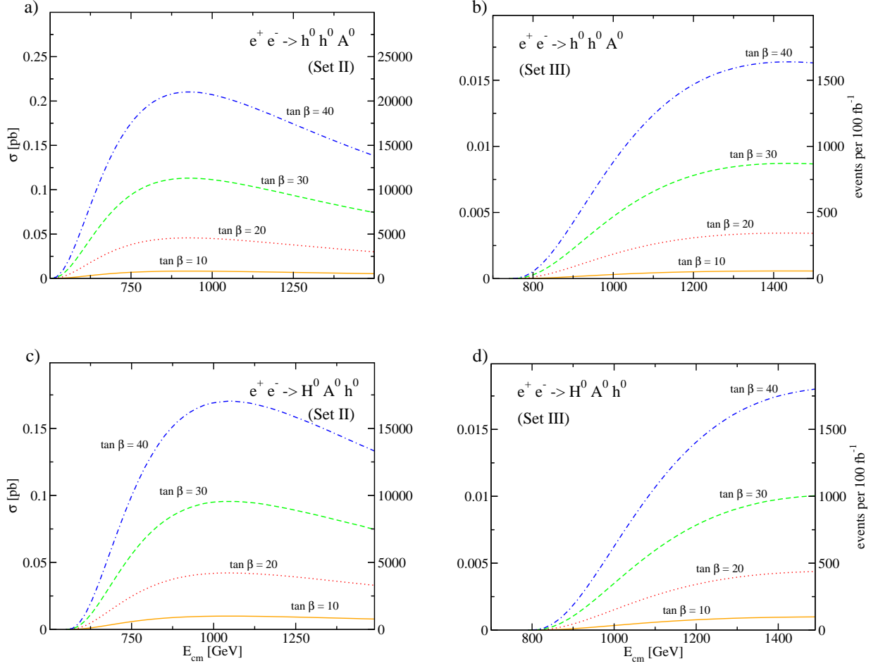
Figure 4: As in Fig. 3, but for processes e^+ e^- \rightarrow h^0 h^0 A^0 and e^+ e^- \rightarrow H^0 A^0 h^0 .
