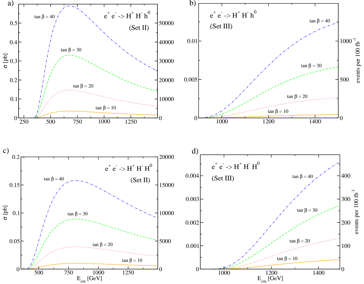
Figure 3: Total cross section \sigma(\text{pb}) and number of events per 100 \text{ fb}^{-1} for the triple Higgs boson production processes e^+e^- \rightarrow H^+H^-h^0 and e^+e^- \rightarrow H^+H^-H^0 in the general 2HDM as a function of \sqrt{s} and for different values of \tan\beta . In each case the label of the process and the choice (Set II or Set III) of Higgs boson masses used for the calculation is indicated, see Table 2.
