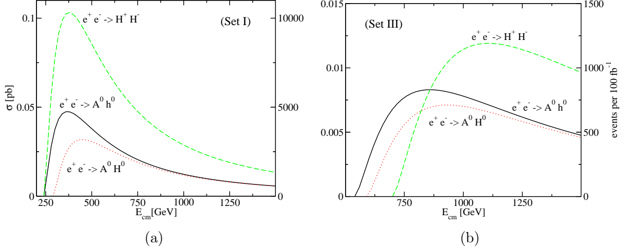
Figure 2: Total cross section \sigma (in pb) and number of events per 100 \text{ fb}^{-1} as a function of E_{\text{cm}} = \sqrt{s} for the tree-level Higgs boson pair production channels (1.1) in the general 2HDM within two regimes of masses: a) light Higgs bosons and b) heavy Higgs bosons, represented by the mass Sets I and III respectively in Table 2.
