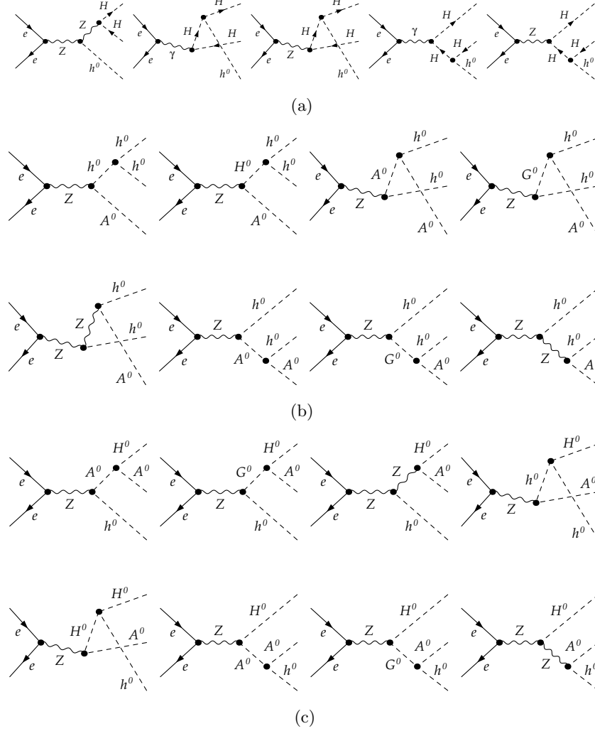
Figure 1: Tree-level Feynman diagrams corresponding to three of the triple Higgs boson production processes indicated in Eq. (1.2). The other four processes proceed through similar collections of diagrams.
