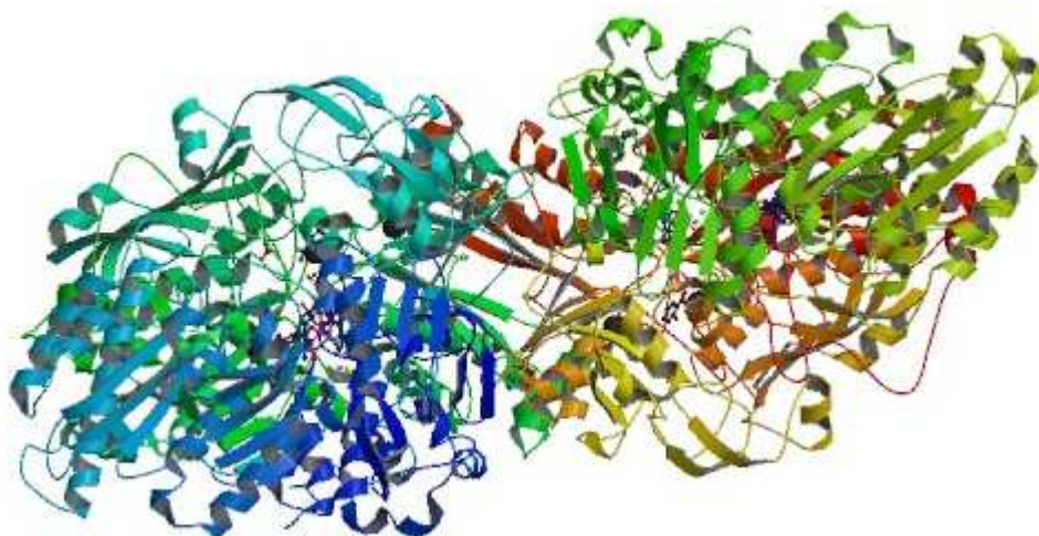
Figure 8. 3D structure of xanthine oxidase.
