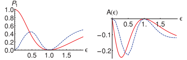
FIG. 4. (Color online) Left: steady-state probability as a function of \epsilon for N = 2 (red) and N = 3 (blue dashed). Right: negative eigenvalue of the partially transposed state as a function of \epsilon for N = 2 (red) and N = 3 (blue dashed). In the N = 3 case, we have set \kappa = 0.8g .
