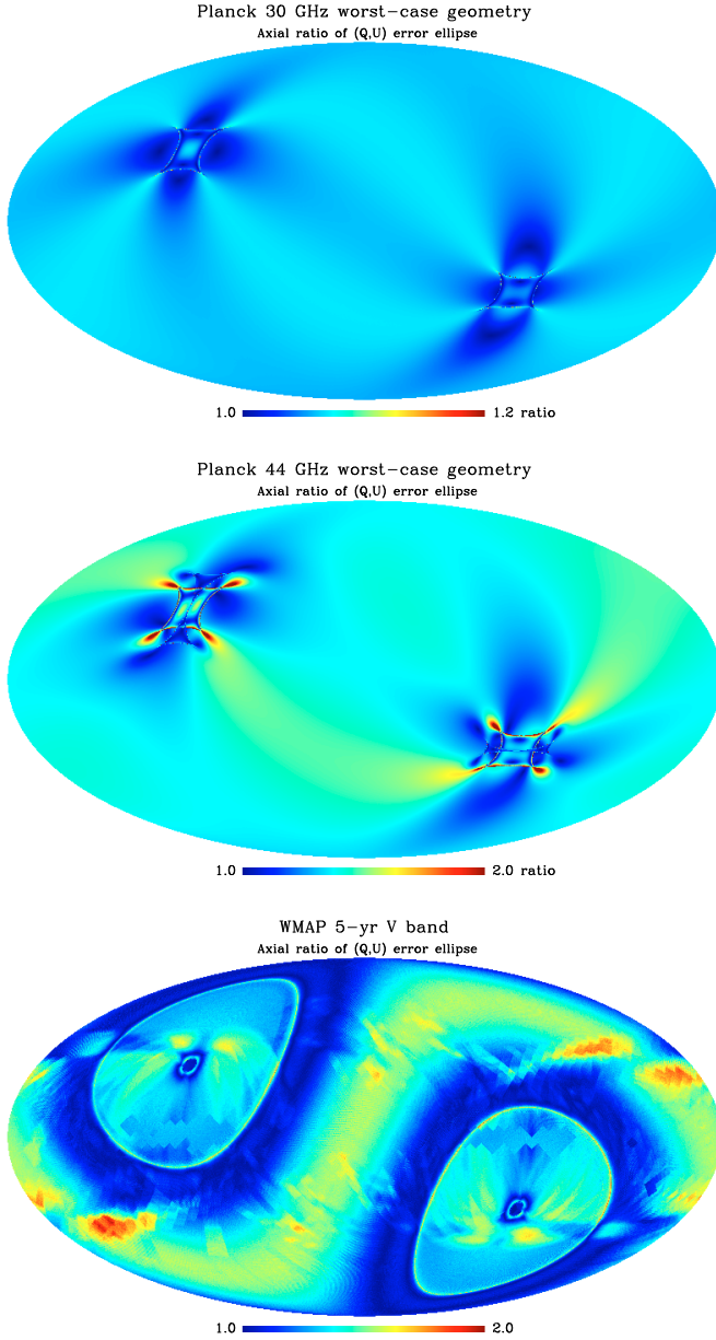
Fig. 11. Simulated pattern on the sky for the axial ratio of the (Q, U) error ellipse for worst-case geometric assumptions at 30 GHz ( top ) and 44 GHz ( middle ). Note that the colour scale for 30 GHz covers only 20% of the range for 44 GHz. Maps are in galactic coordinates. The actual pattern for the WMAP 5-year V band is show at bottom, on the same colour scale as for Planck at 44 GHz.
