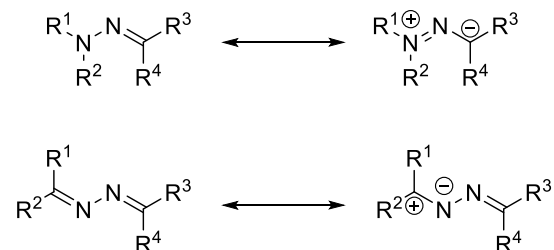
Fig. 1. Resonance structures for hydrazones and azines.
