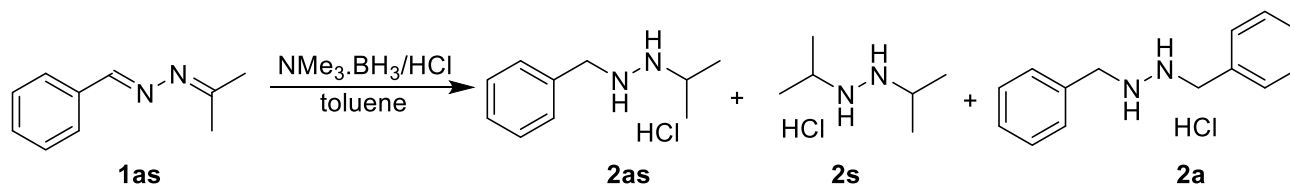
Scheme 3. Reduction of azine 1as.
