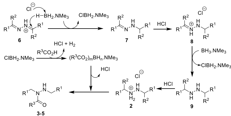
Scheme 4. A plausible mechanism for the reduction and acylation of azines.
