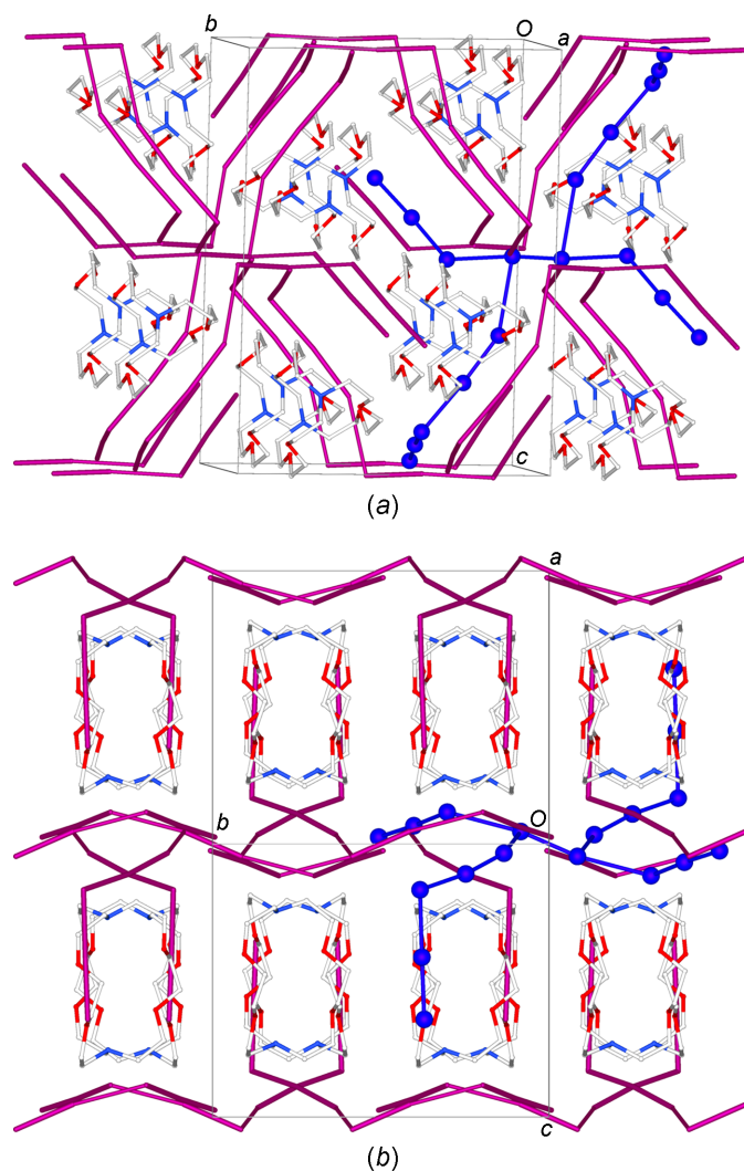
Figure 9 Views along approximately (a) the a axis and (b) the [101] direction of the crystal packing in (II). The blue colour and the ball-and-stick representation have been used for one of the discrete I_{18}^{4-} polyiodide units to better highlight its atomic connectivity in the crystal packing. H atoms and the cocrystallized CH_2Cl_2 molecules are not shown.
