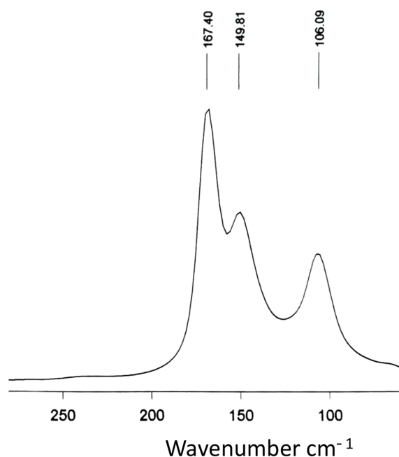
Figure 10 FT-Raman spectrum of (II) in the low frequency region.
