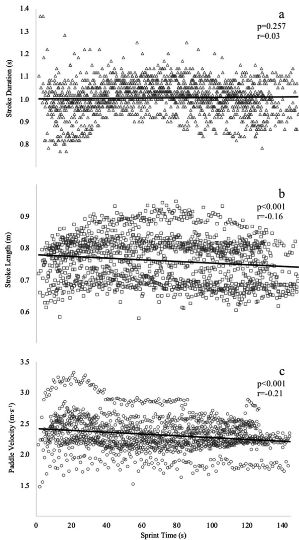
Figure 2. Scatter plots between sprint time and (a) stroke duration (triangles); (b) stroke length (squares) and (c) paddle velocity (circles). The solid lines represent the regression lines of each scatter plot.
