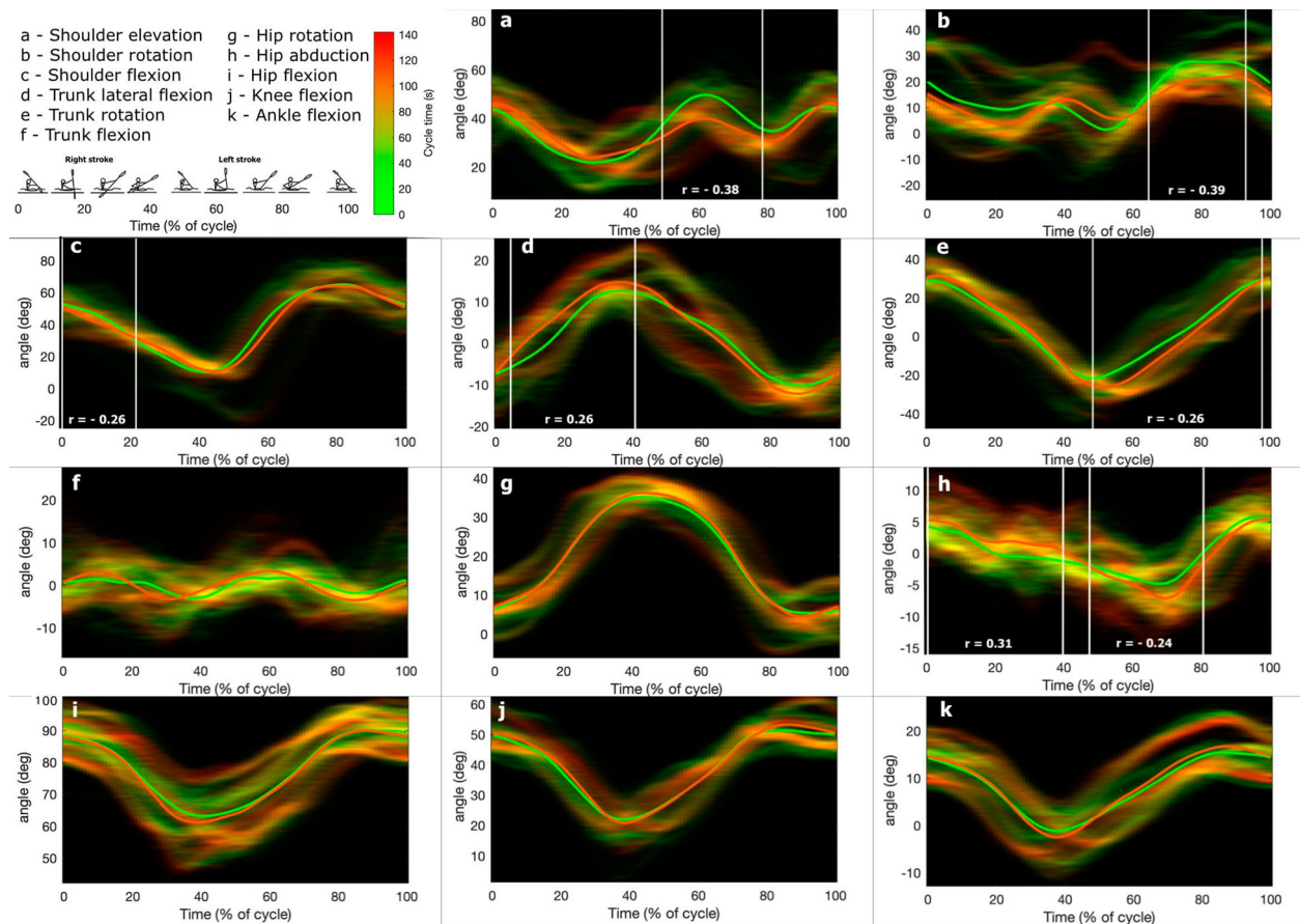
Figure 3. Group mean curves of joint angles normalized to the duration (0–100%) of the stroke cycle. (a) Shoulder elevation, (b) shoulder rotation, (c) shoulder flexion, (d) trunk lateral flexion, (e) trunk rotation, (f) trunk flexion, (g) hip rotation, (h) hip abduction, (i) hip flexion, (j) knee flexion and (k) ankle flexion. Mean curves are presented for the initial (cycles 11–20) and ending part (last 10 cycles) of the sprint trial (green and red lines, respectively). Line density around the means represents the kinematic change over time: colors code refers to the time within the test when each cycle occurred. The x-axis value 0% represents the beginning of the pull phase on the right side and 100% represents the return to the beginning of the same phase on the ipsilateral side. The white vertical lines represent the start and the end of each phase in which a significant correlation with race time was found (significant cluster, Statistical Parametric Mapping, p < .05 ).
