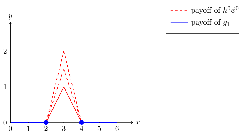
Figure 3: h^0 \phi^0 does not dominate g_1 on (K_0, K_0 + \varepsilon) for any h^0 with \varepsilon = \varepsilon(h^0)
