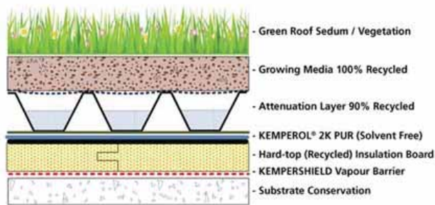
KEMPERGRO® Green Roof System Build Up
