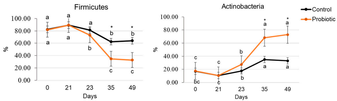
Day ( p < 0.001 ), S ( p < 0.001 ), Day \times S ( p < 0.001 ) Day ( p < 0.001 ), S ( p < 0.001 ), Day \times S ( p < 0.001 )
