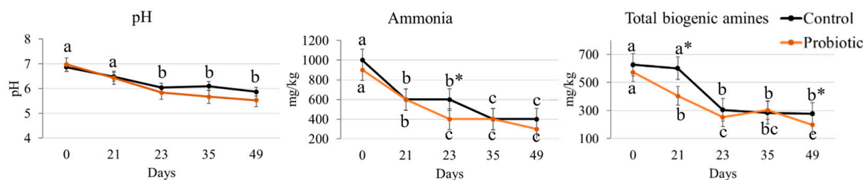
Day ( p < 0.001 ), S ( p = 0.01 ), Day \times S ( p = 0.08 ) Day ( p < 0.001 ), S ( p < 0.001 ), Day \times S ( p = 0.01 ) Day ( p < 0.001 ), S ( p < 0.001 ), Day \times S ( p = 0.04 )
