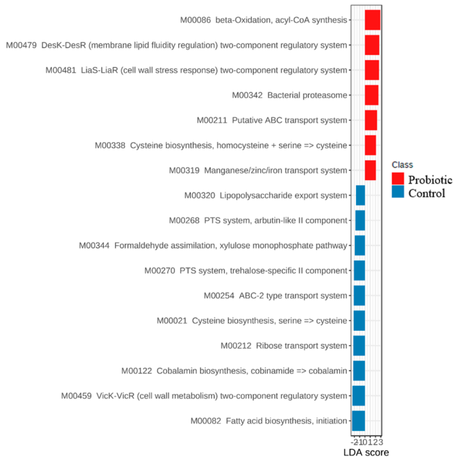
Figure 6. LDA score of modules that statistically differ ( p < 0.05 ) between the control and probiotic groups fed the lower protein and fiber diet—day 21 (A) and the higher protein and fiber diet—day 49 (B).
