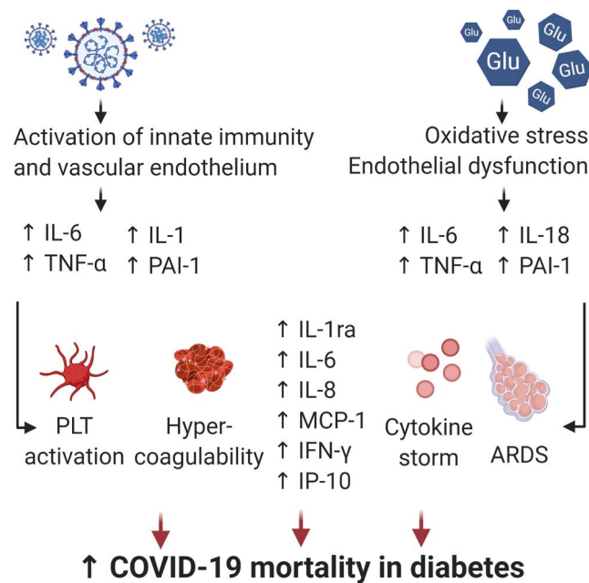
FIGURE 5 Excessive inflammation and vascular dysfunction are a key feature of both hyperglycemia and COVID-19, making up the ground for a detrimental synergistic combination. The increase of IL-1ra, IL-6, IL-8, MCP-1, IFN- \gamma , and IP-10 observed in subjects with type 2 diabetes and COVID-19 may contribute to explain the greater disease severity observed in diabetic patients
