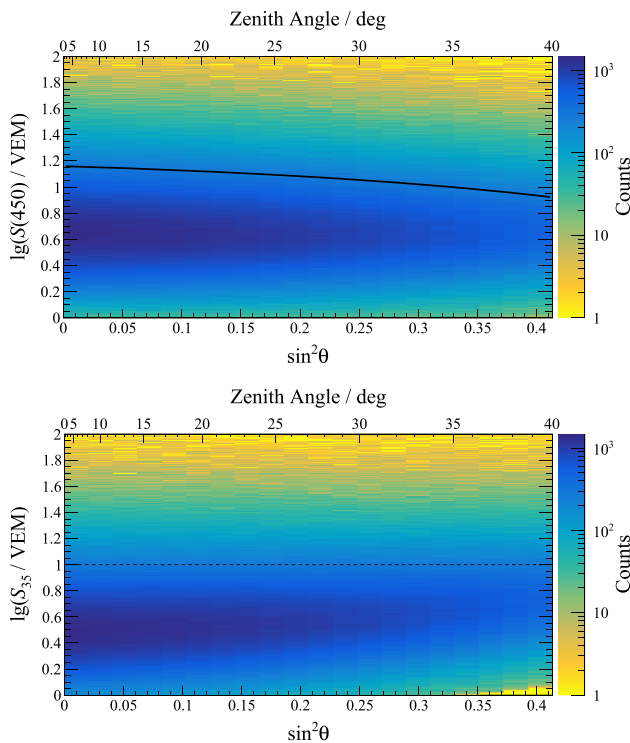
Fig. 6 Top: histogram of reconstructed shower sizes and zenith angles. The solid black line represents the shape of f_{CIC} at 10 VEM. Bottom: same distribution but as a function of corrected shower size, S_{35} , and zenith angle. The dashed black line indicates the mapping of the solid black line in the top figure after inverting the effects of the CIC correction
