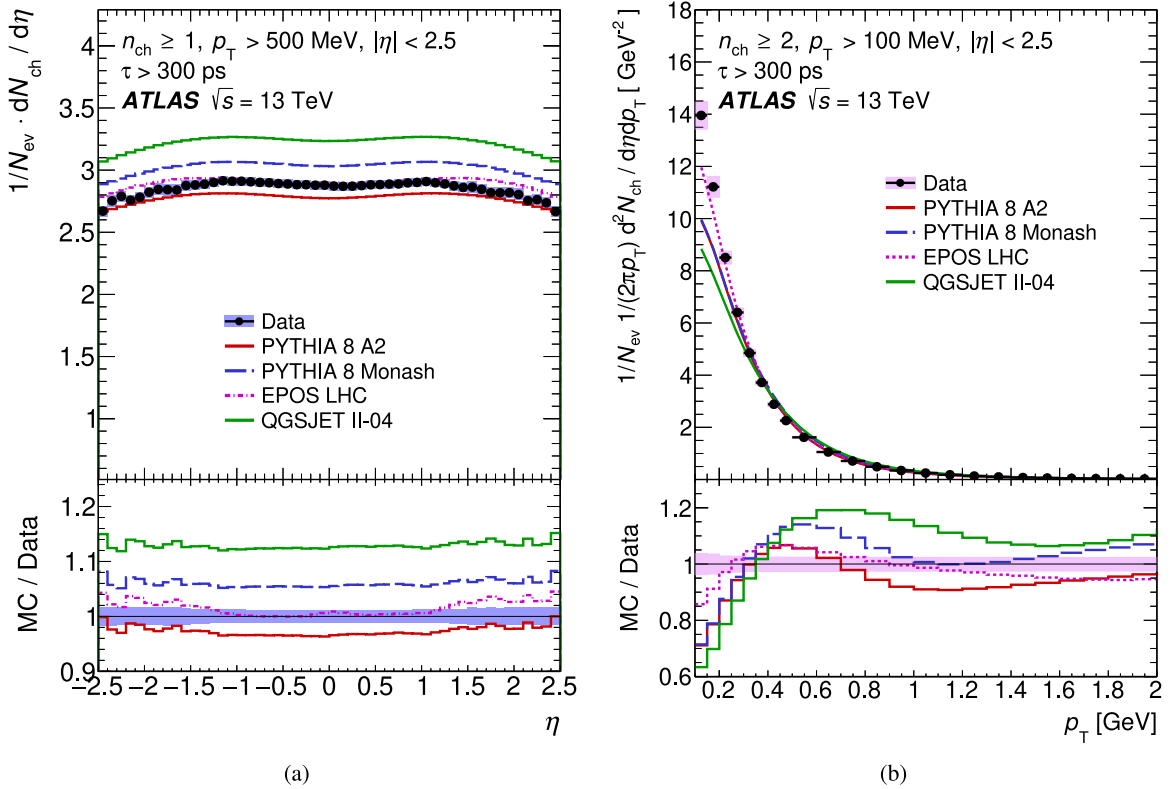
Fig. 5. (a) Primary charged-particle multiplicities as a function of pseudorapidity in events with at least one primary charged particle with p_T > 500 MeV and |\eta| < 2.5 [56]. (b) Primary charged-particle multiplicities as a function of transverse momentum in events with at least two primary charged particles with p_T > 100 MeV and |\eta| < 2.5 [57]. The dots represent the data and the curves the different MC model predictions. The lower panels show the ratios of the predictions to the data.
