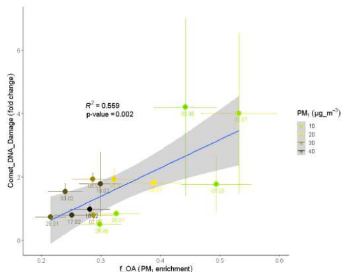
Fig. 6. Exposure-response curves of A) Comet assay ( n = 14 ) results vs the enrichment of PM_1 in organic aerosol (OA). The Comet-OA curve, statistically significant, and with a high R^2 = 0.559 , underline the relevance of the chemistry determining atmospheric aerosol toxicological properties rather than the airborne mass, number, or surface area exposure doses. Noteworthy, higher DNA damaging effects were related to low PM_1 airborne concentrations.
