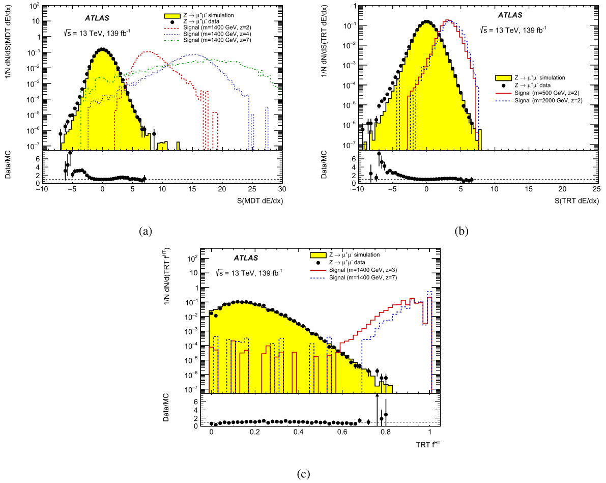
Fig. 3. Normalized distributions of the dE/dx significance in (a) the MDT, S(\text{MDT } dE/dx) , (b) the TRT, S(\text{TRT } dE/dx) , and (c) of TRT f^{\text{HT}} for muons from Z \rightarrow \mu\mu events (data and simulation) and for simulated MCPs passing preselection requirements. Bin-by-bin ratios of Z \rightarrow \mu\mu distributions in data and simulation are shown on the lower panels. The arrow in the ratio plot in (c) is for a point that is outside the range.
