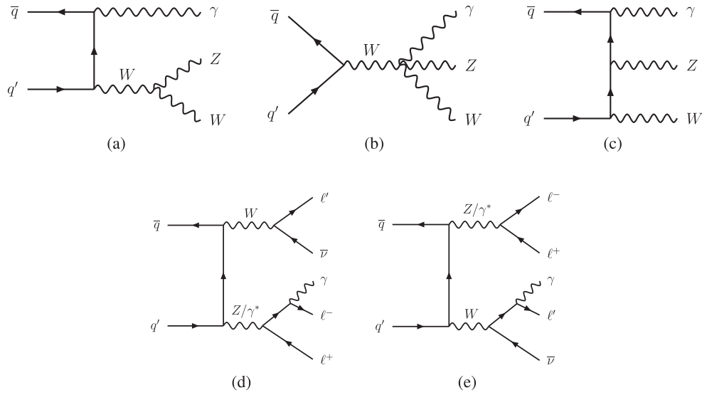
FIG. 1. Representative leading-order Feynman diagrams for (a)–(c) WZ\gamma production and (d),(e) \ell'^{\pm}\nu\ell^{+}\ell^{-}\gamma production via the FSR processes Z \rightarrow \ell^{+}\ell^{-}\gamma and W \rightarrow \ell'\nu\gamma .
