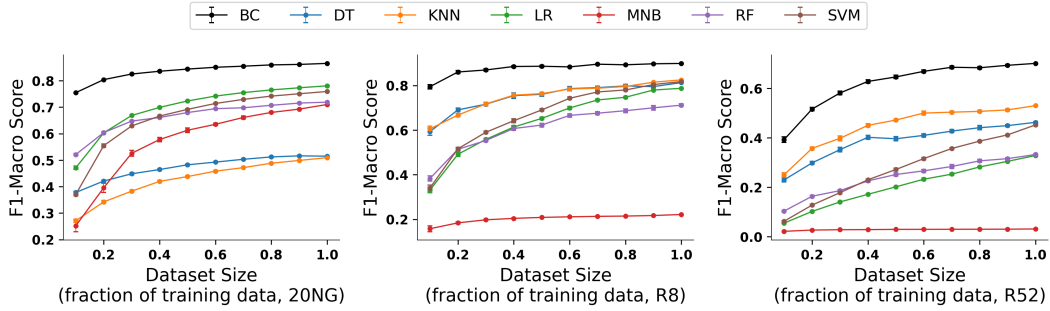
Figure 3: F1-macro score (y-axis) on 20Newsgroup, R8, R52, for several classifiers, in function of the fraction of data used for training (x-axis).
