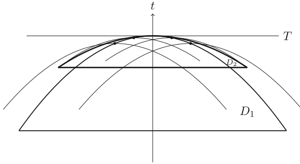
Fig. 1 An illustration of the first two parabolic regions D_j : the region D_2 is a subset of the union of D_1 with suitable parabolic regions \tilde{D}^{(x_0,t_0)} having vertices at points (x_0, t_0) \in \partial D_1 (black dots in the graph). The region D_3 will be a subset of the union of D_2 with parabolic regions \tilde{D}^{(x_0,t_0)} having vertices at points (x_0, t_0) \in \partial D_2 . As j grows, the opening of the regions D_j increases, as it is defined by the parameter \sigma_j \uparrow \infty . The union of the regions D_j contains the cylinder B_{1/2}^k \times [-1/4, 0) , over which we can conclude graphical parametrization and corresponding estimates for the flow
