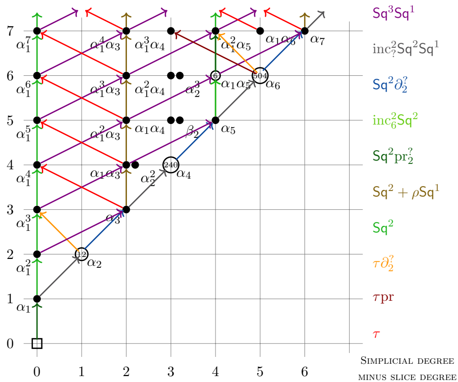
Figure 3.1: The first slice differential for 1_\Lambda .
