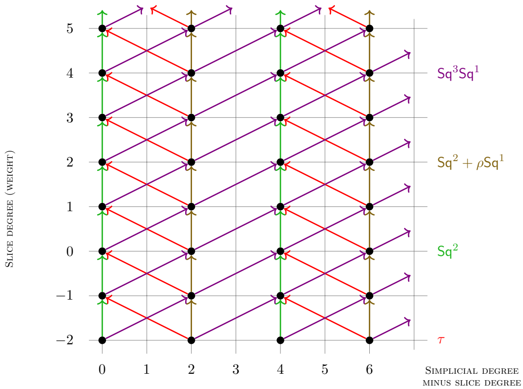
Figure 2.2: The first slice differential for \mathbf{k}w .
