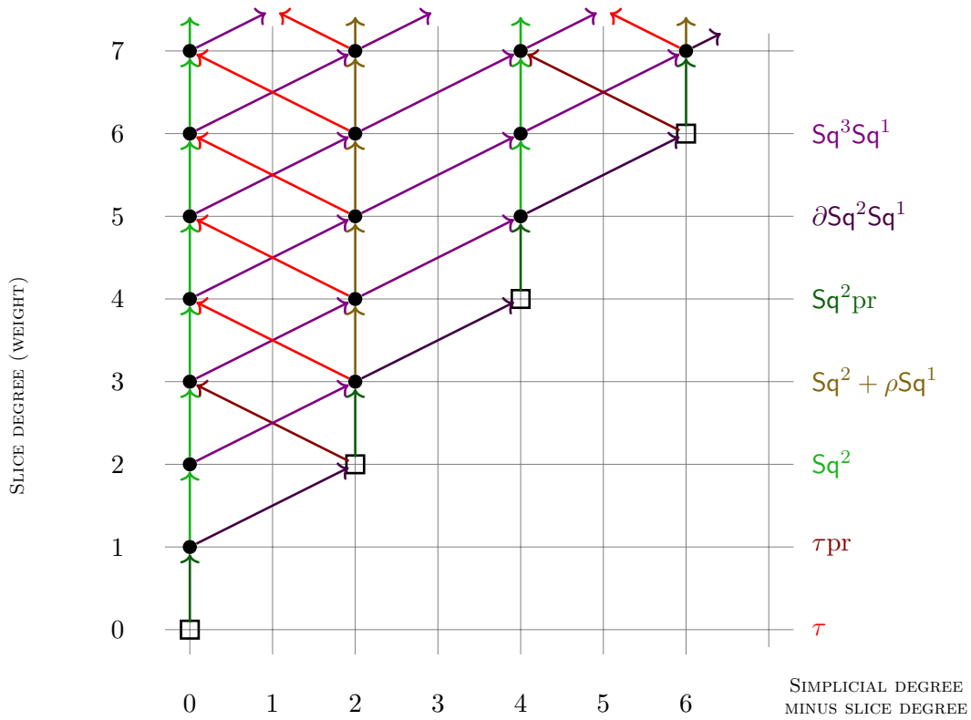
Figure 2.1: The first slice differential for kq .
