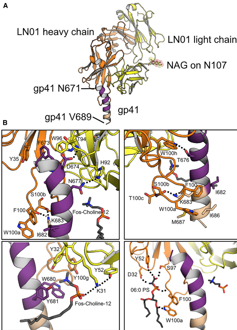
Figure 5. Structure of LN01 in Complex with gp41 MPER-TM1 and with Lipid
