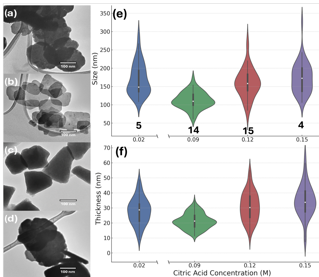
Figure 5. TEM images of NS5, NS14, NS15 and NS4 ((a), (b), (c), (d), respectively) and dimensions (e) and thickness distributions (f). The distributions shown represent the mean square average diameter (MSA).
