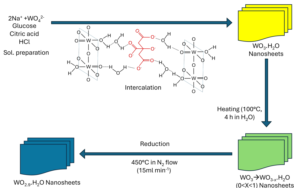
Figure 4. Proposed mechanism of \text{H}_2\text{WO}_4 nanosheet production [31].
