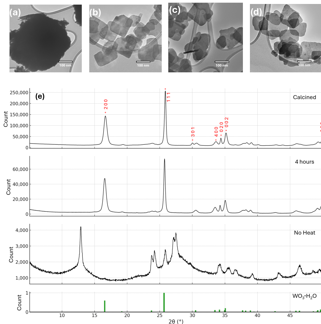
Figure 1. TEM of nanosheets resulting from NS13 with no citric acid (a) and NS14 with 1 h of stirring but no heating phase (b), after 4 h of heating (c) and after reduction in \text{N}_2 (d). Below (e), comparison of XRD results for each obtained nanosheet sample, with the reference of \text{WO}_3 \cdot \text{H}_2\text{O} at the bottom.
