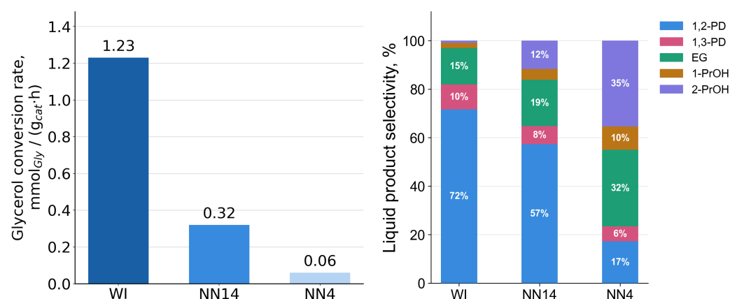
Figure 8. Left: Average glycerol conversion rates of WI, NN14 and NN4 catalysts. Right: Liquid product selectivity of WI, NN14 and NN4 catalysts.
