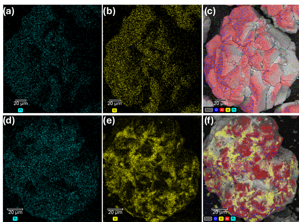
Figure 7. SEM-EDS images of the \text{Pt}/\text{WO}_3/\text{Al}_2\text{O}_3 WI (a–c) and NN14 (d–f) catalysts after 500 °C calcination and three washes with a centrifuge, using 300 mL of Milli-Q water for each wash. Each element is represented by a color: O = blue, W = yellow, Al = red, Pt = cyan.
