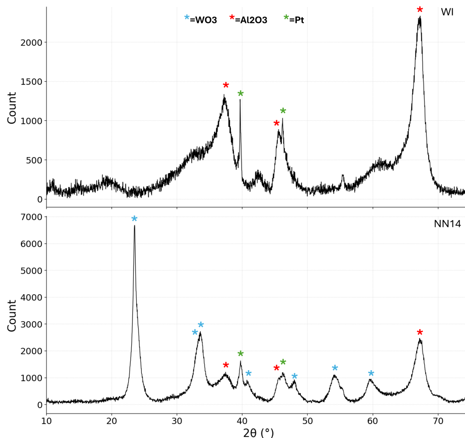
Figure 6. XRD patterns of the WI (top) and NN14 (bottom) catalysts after 500 °C calcination and pre-reduction. Asterisks indicate diffraction peaks attributed to \gamma\text{-Al}_2\text{O}_3 (red), Pt (green) and monoclinic \text{WO}_3 (blue, NN14 only).
