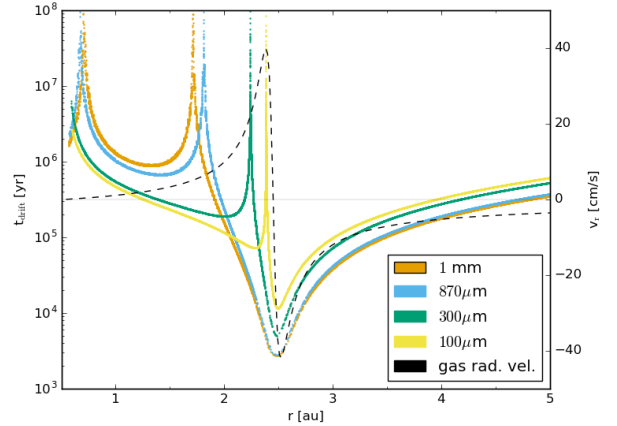
Figure 1. The drift timescales of the dust particles of different sizes are plotted at the location and at the time of gap opening. The radial velocity of the gas is overplotted with a dashed line and its zero value is marked with a grey line.
